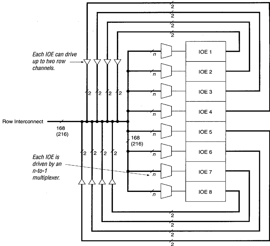
Figure 11. FLEX 8000 Row-to-IOE Connection
