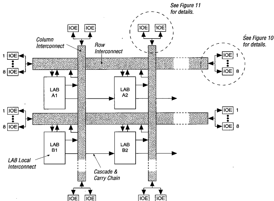
Figure 9. FLEX 8000 Device Interconnect Resources
