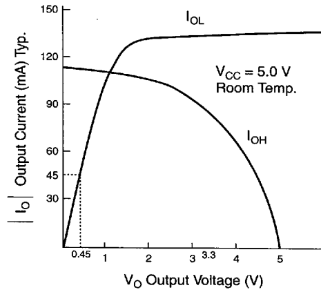
Figure 16. Output Drive Characteristics of EPF8282A Devices with 5.0-V V_{CCIO}
