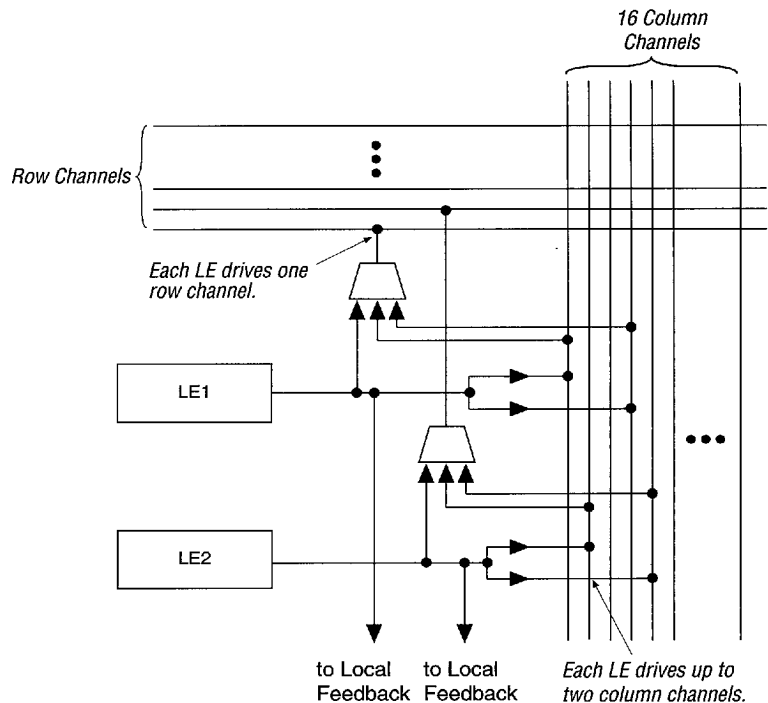
Figure 8. LAB Connections to Row & Column Interconnect
