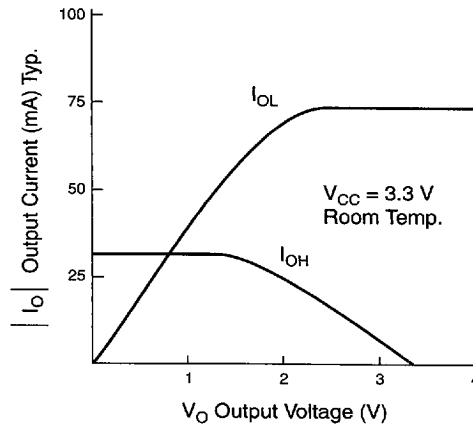
Figure 17. Output Drive Characteristics of EPF8282AV Devices
