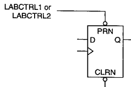
Figure 7. LE Asynchronous Clear & Preset Modes
