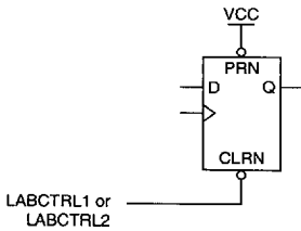
Figure 7. LE Asynchronous Clear & Preset Modes
