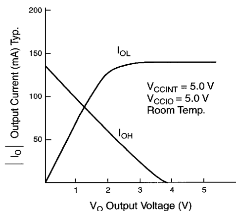
Figure 15. Output Drive Characteristics of 5.0-V Devices (except EPF8282A)
