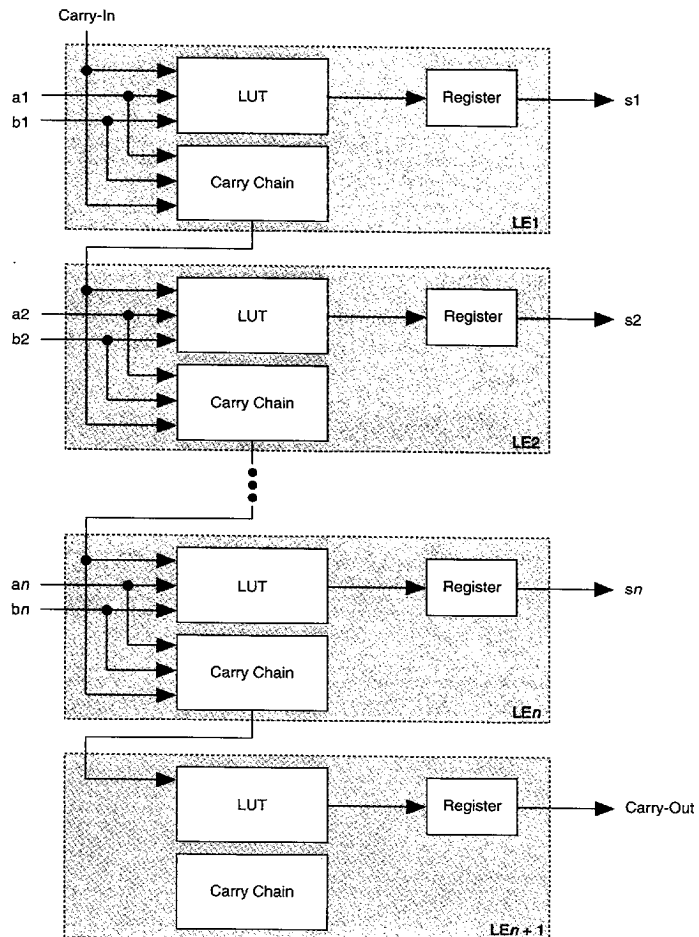
Figure 4. Carry Chain Operation
