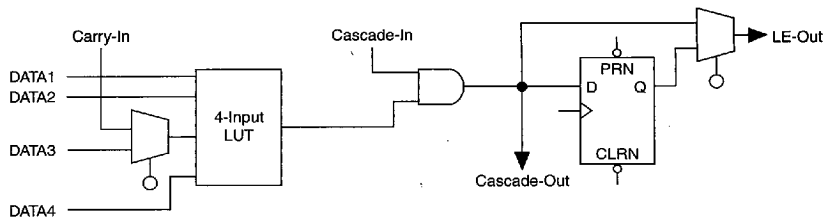
Figure 6. FLEX 8000 Logic Element Operating Modes
