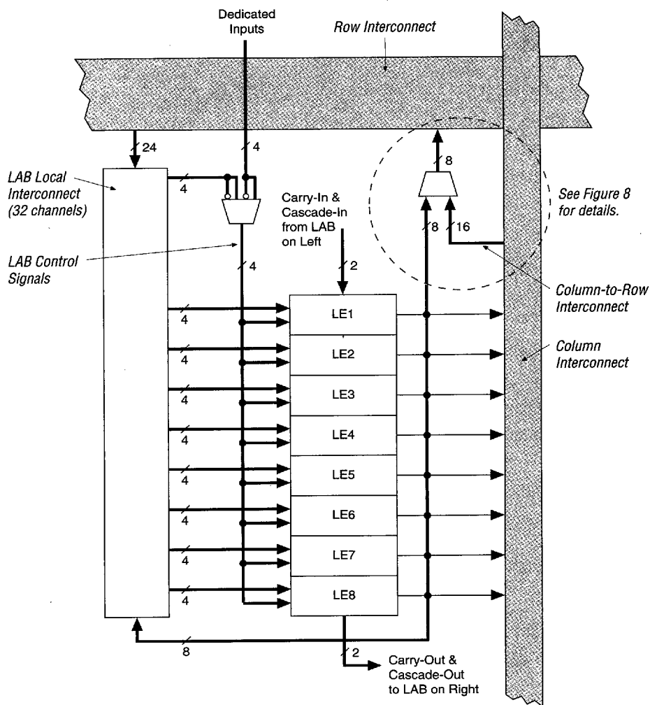
Figure 2. FLEX 8000 Logic Array Block
