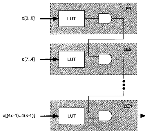
AND Cascade Chain
