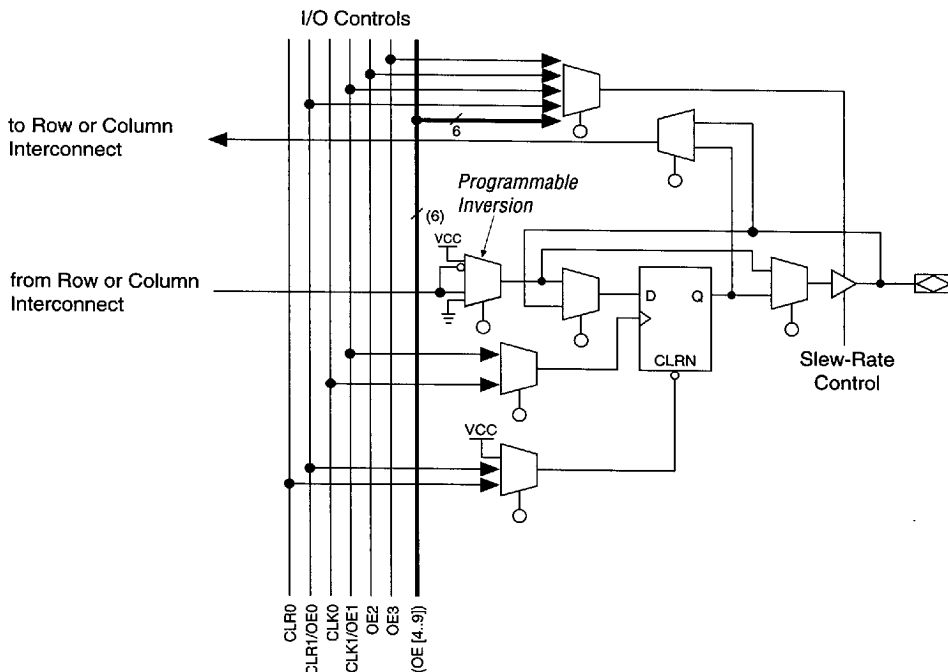
Figure 10. I/O Element (IOE)
