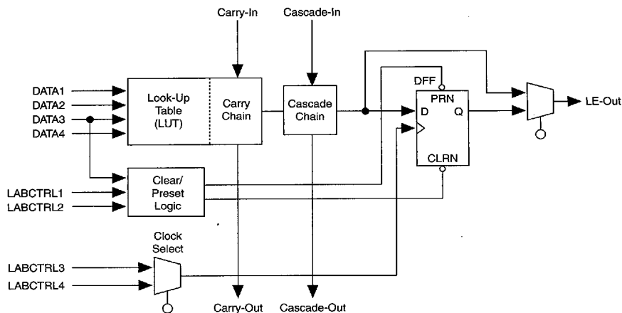
Figure 3. FLEX 8000 Logic Element (LE)
