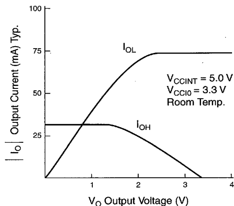
Figure 15. Output Drive Characteristics of 5.0-V Devices (except EPF8282A)
