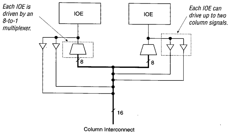
Figure 12. FLEX 8000 Column-to-IOE Connection
