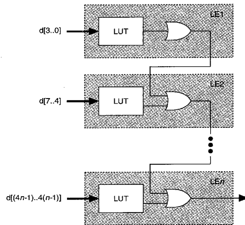
OR Cascade Chain
