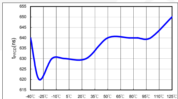
Figure 14. t PFC-D vs. Temperature
