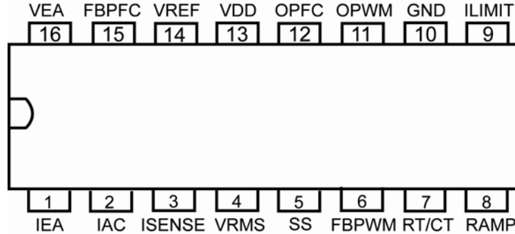
Figure 6. Pin Configuration (Top View)
