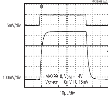
SMALL-SIGNAL TRANSIENT (GAIN = 90V/V)
