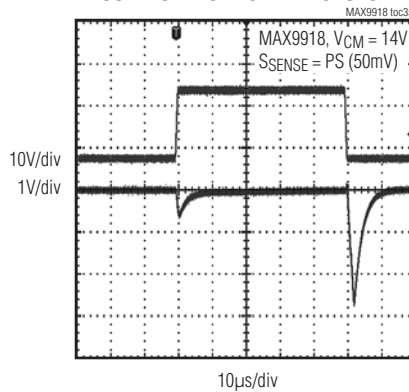
COMMON-MODE STEP RESPONSE
