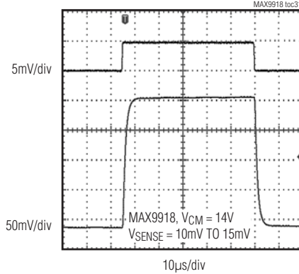
SMALL-SIGNAL TRANSIENT (GAIN = 45V/V)
