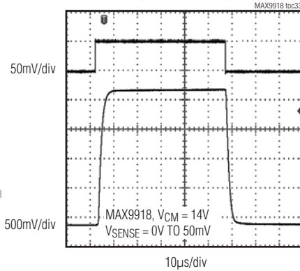
LARGE-SIGNAL TRANSIENT (GAIN = 45V/V)
