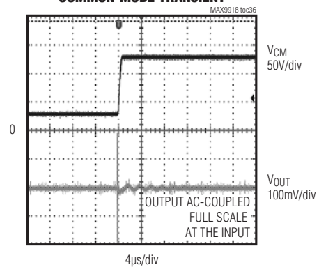
OUTPUT RESPONSE TO COMMON-MODE TRANSIENT
