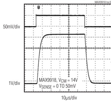
LARGE-SIGNAL TRANSIENT (GAIN = 90V/V)
