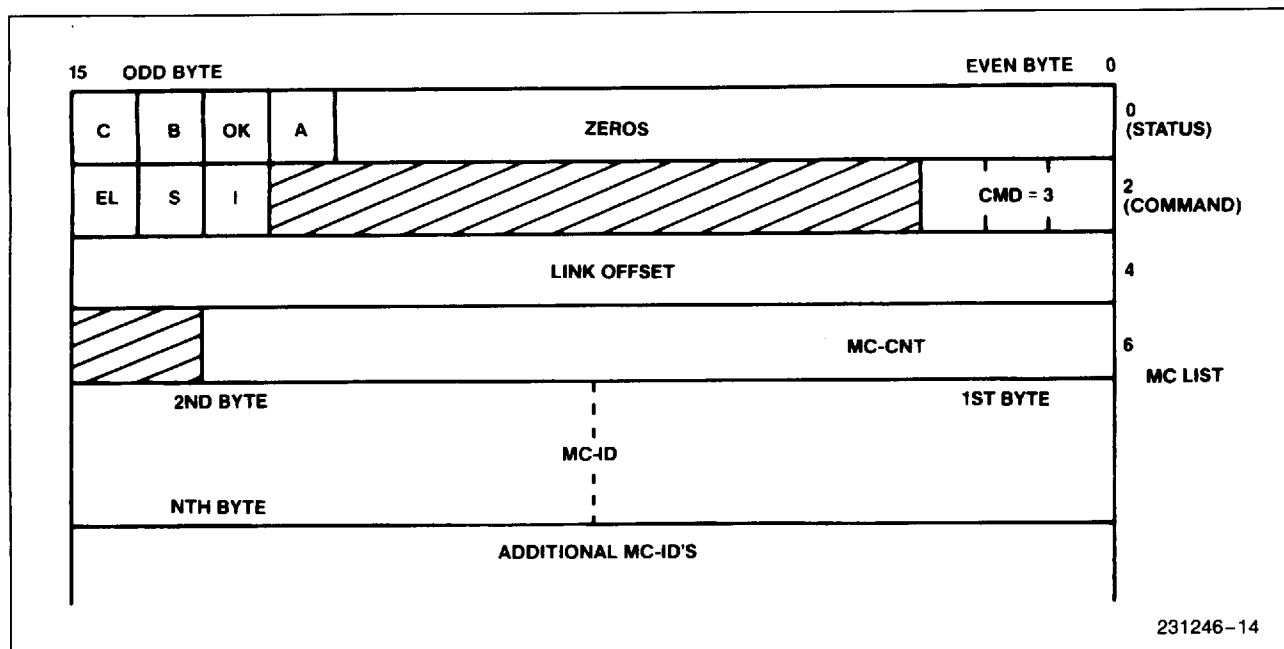
Figure 14. The MC-SETUP Command Block
