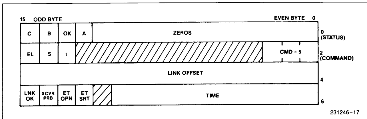
Figure 17. The TDR Command Block
