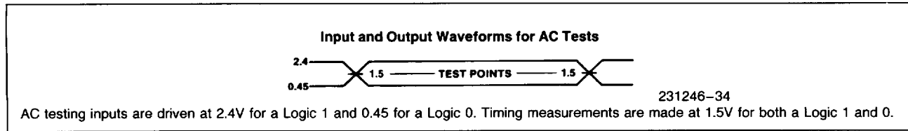
Figure 33. TTL Input/Output Voltage Levels for Timing Measurements
