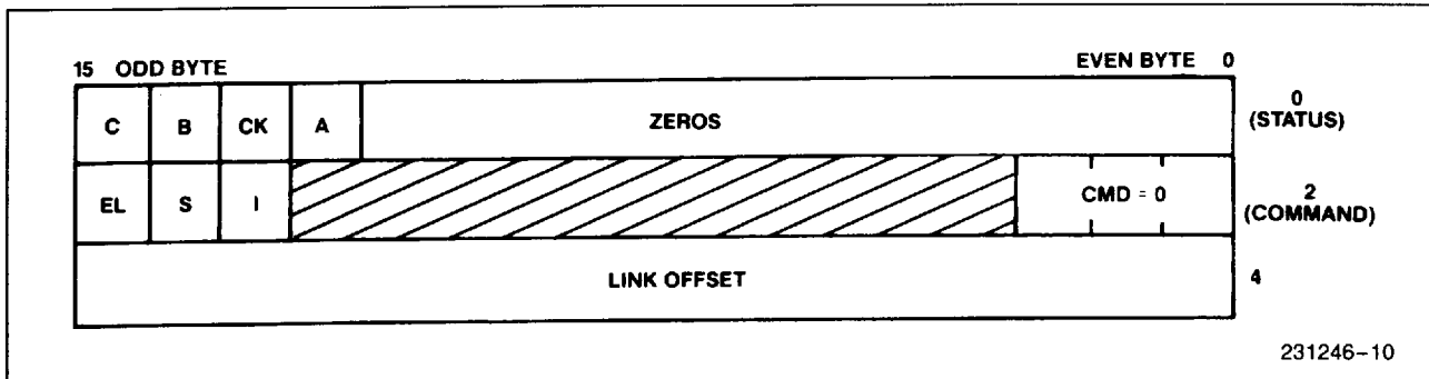
Figure 11. The NOP Command Block
