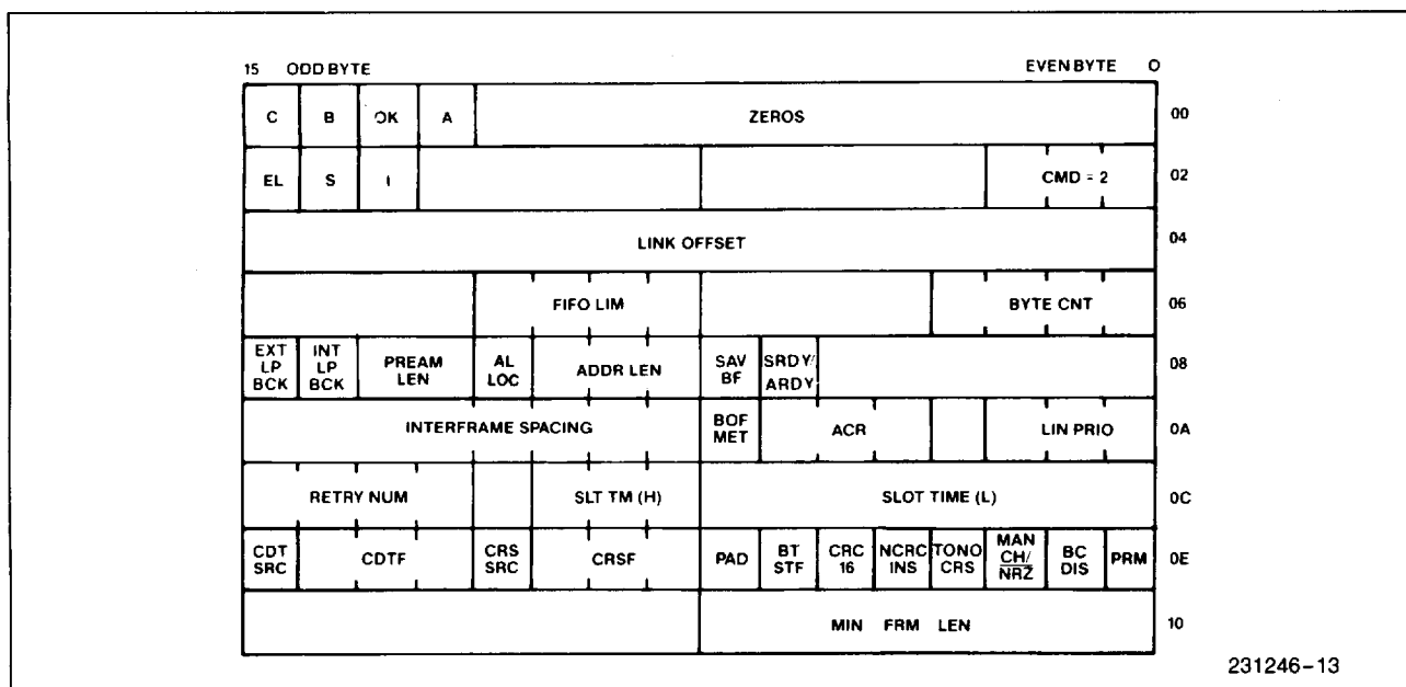
Figure 13. The CONFIGURE Command Block
