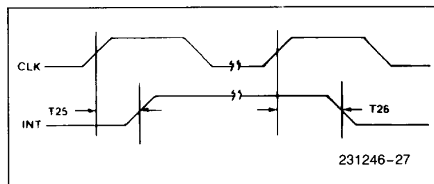
Figure 26. INT Output Timing
