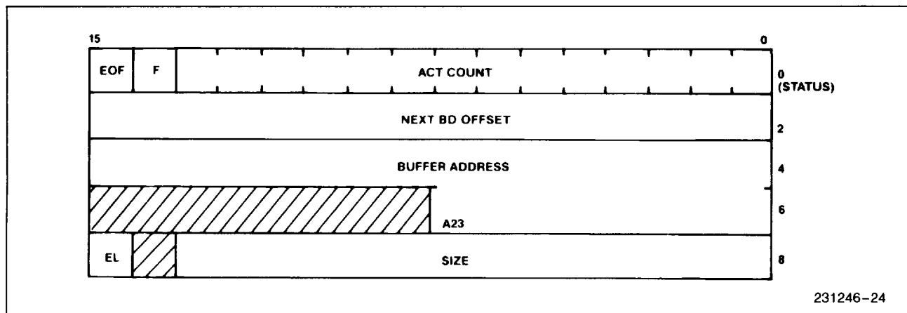
Figure 23. The Receive Buffer Descriptor (RBD) Format
