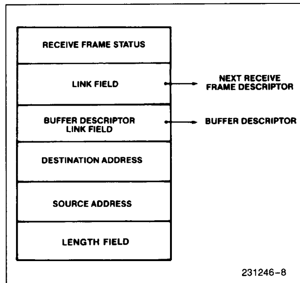
Figure 9. Receive Frame Descriptor
