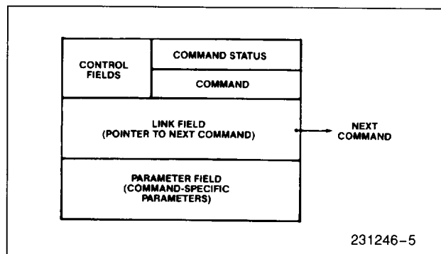
Figure 5. Action Command Format
