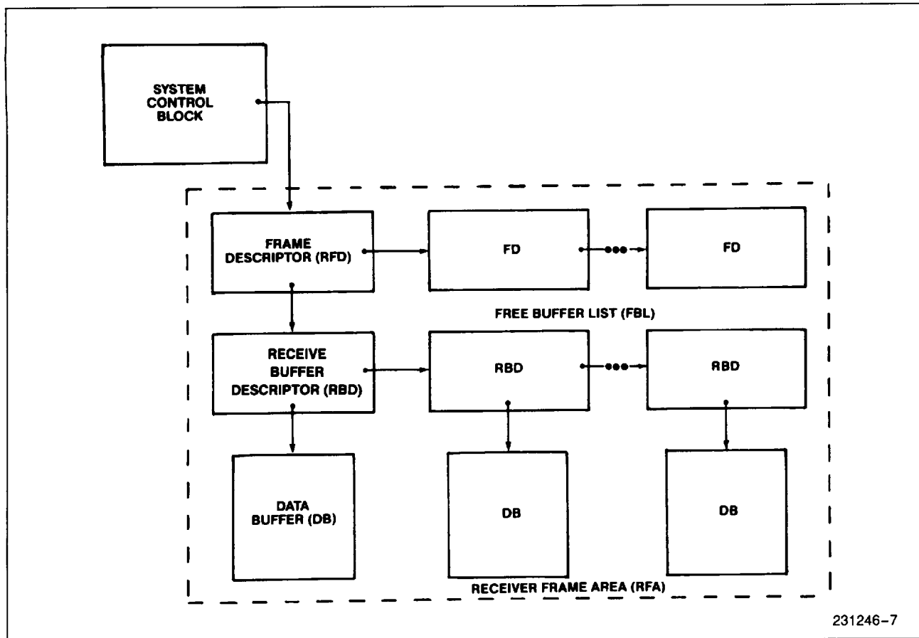
Figure 8. Receive Frame Area Diagram
