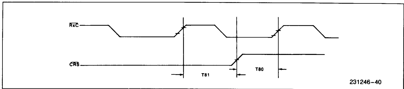
Figure 38. CRS Timing Relative to RxC
