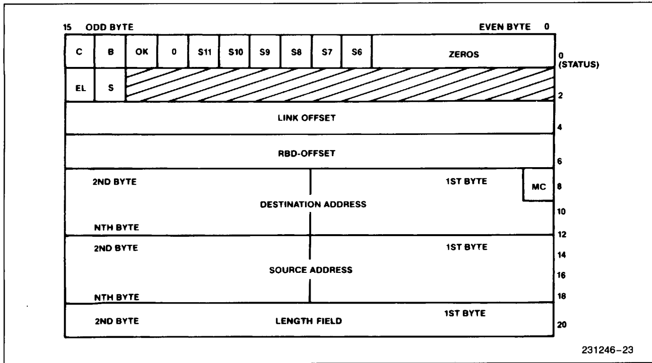
Figure 22. The Frame Descriptor (FD) Format
