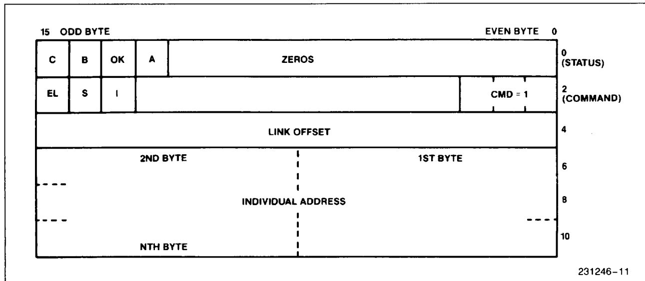
Figure 12. The IA-SETUP Command Block
