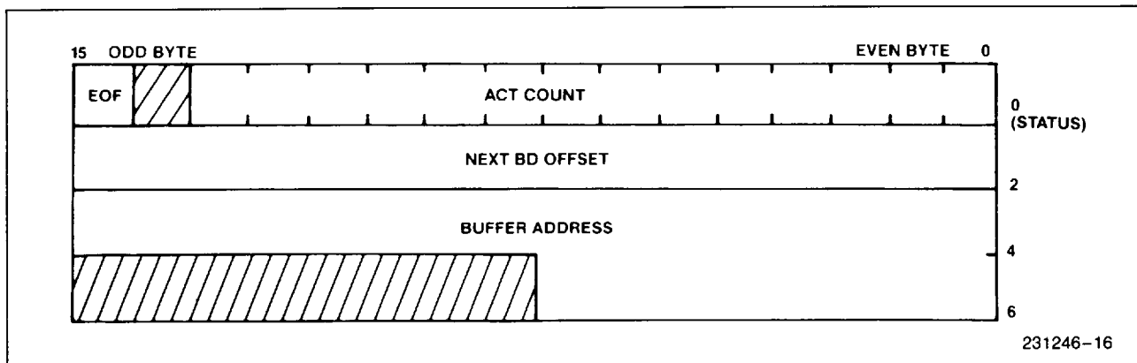
Figure 16. The Transmit Buffer Description
