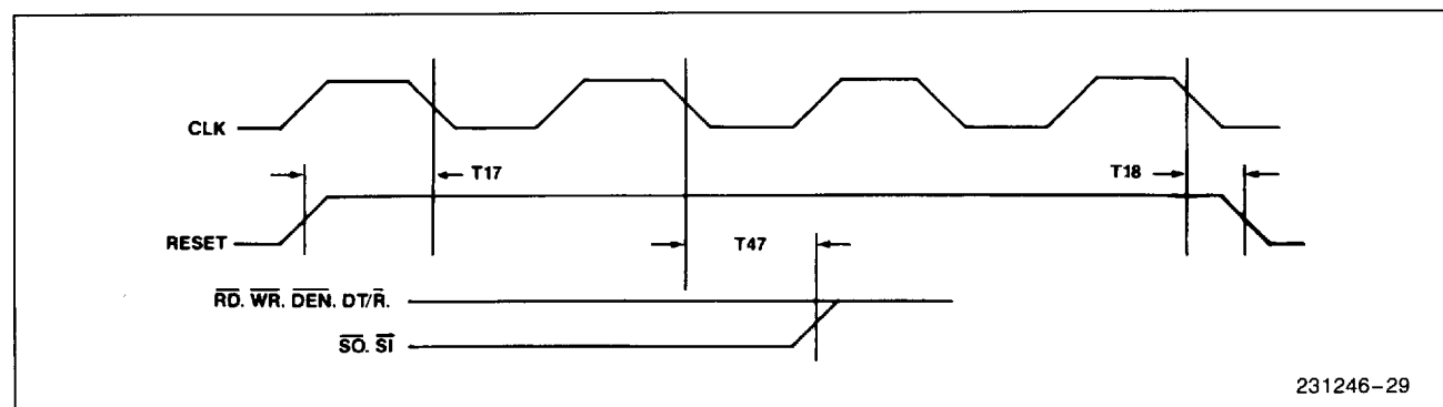
Figure 28. RESET Timing
