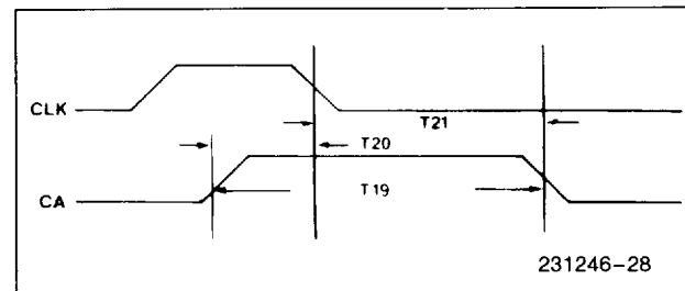
Figure 27. CA Input Timing
