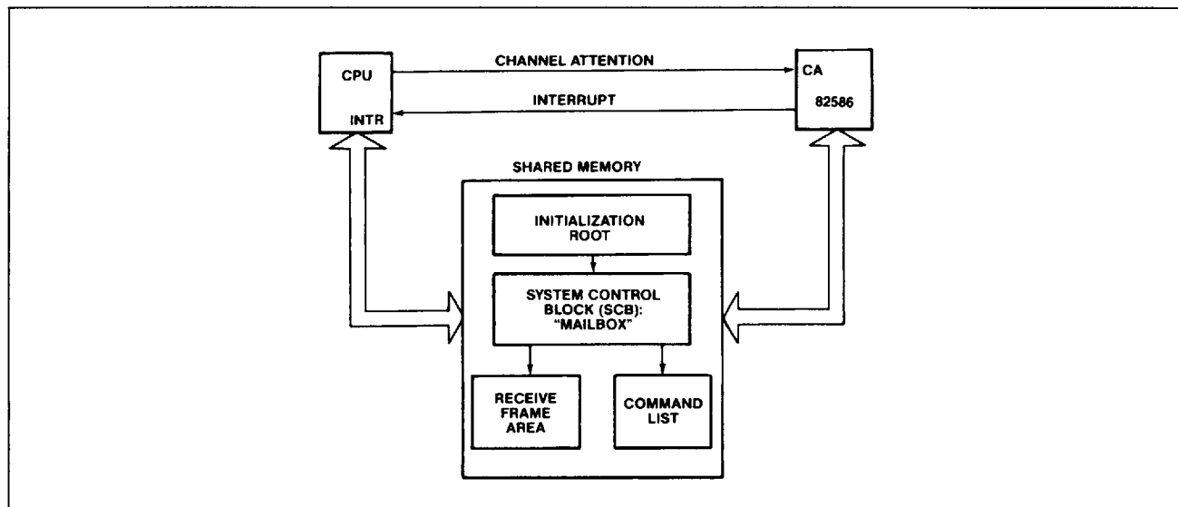
Figure 3. 82586/Host CPU Interaction
