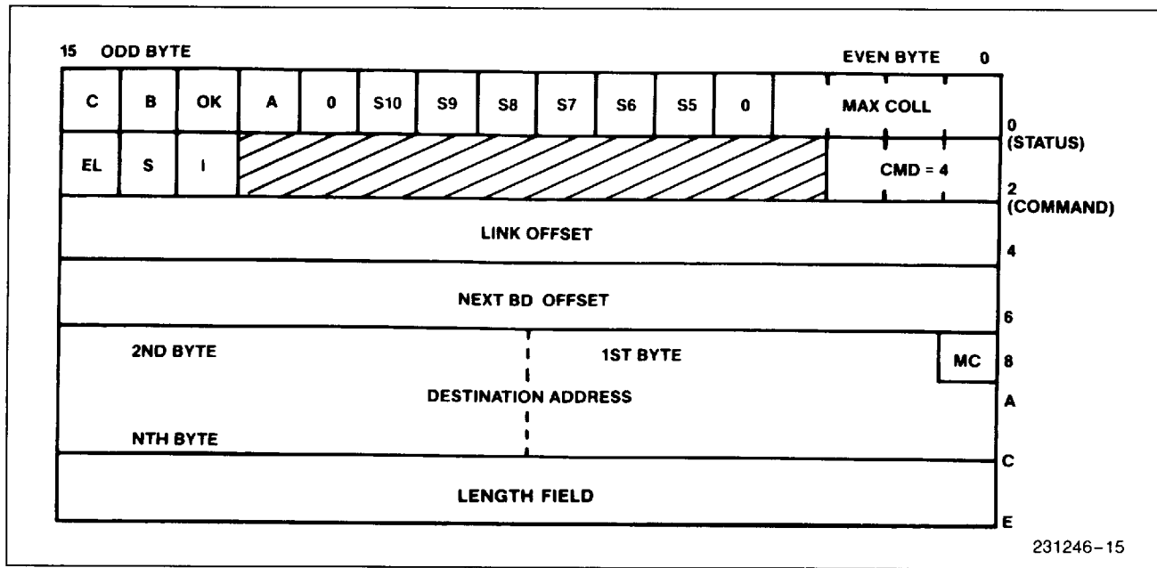
Figure 15. The Transmit Command Block
