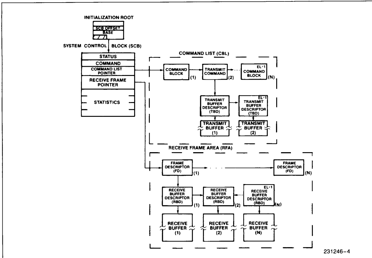
Figure 4. 82586 Shared Memory Structure
