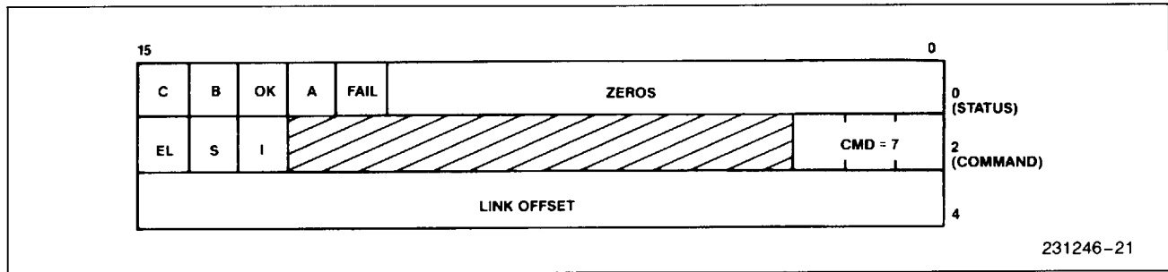
Figure 20. The DIAGNOSE Command Block
