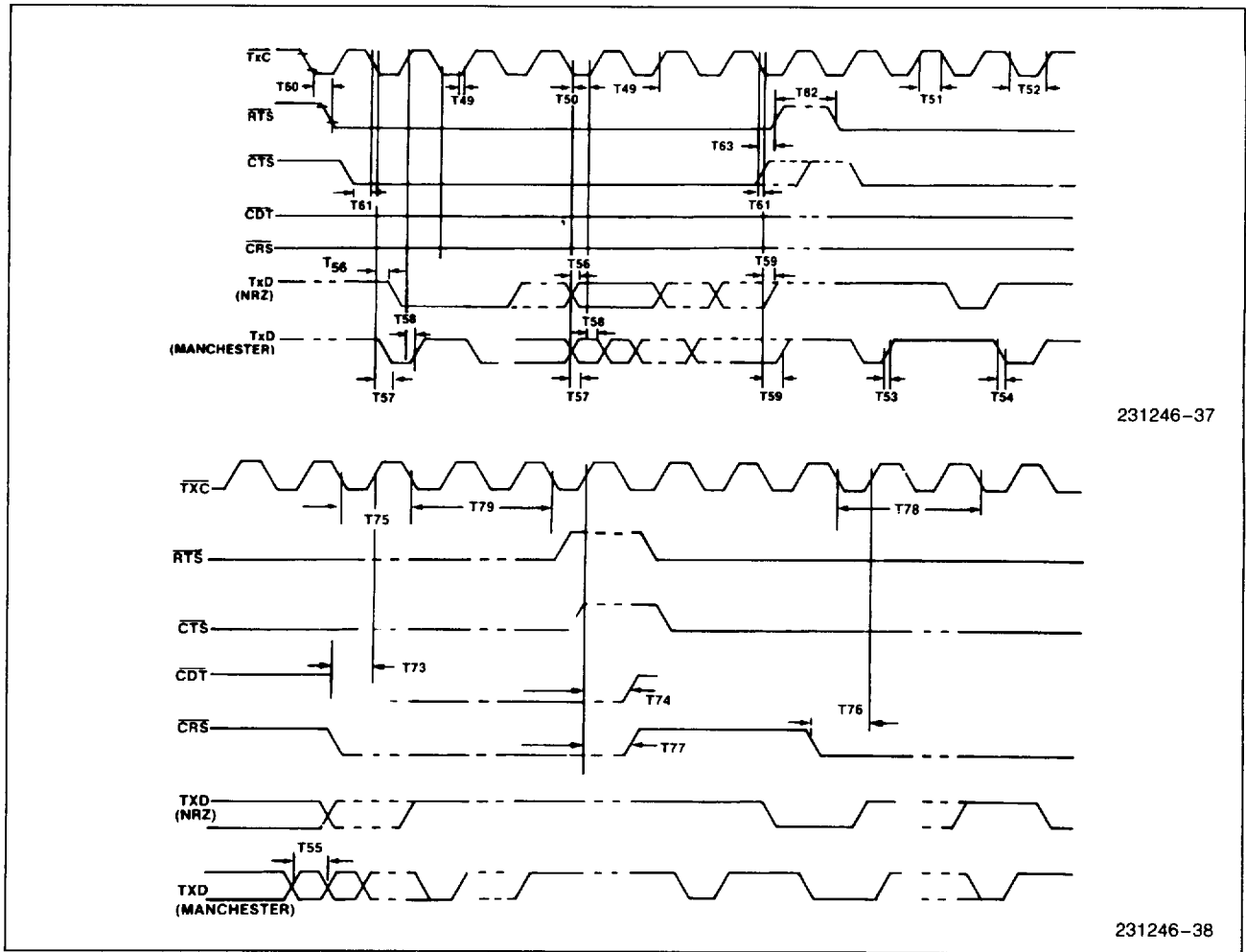
Figure 36. Transmit and Control and Data Timing
