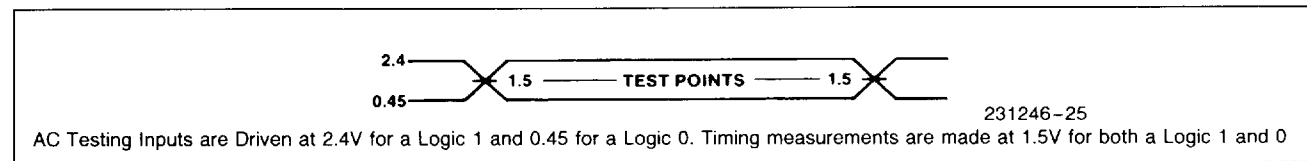
Figure 24. TTL Input/Output Voltage Levels for Timing Measurements
