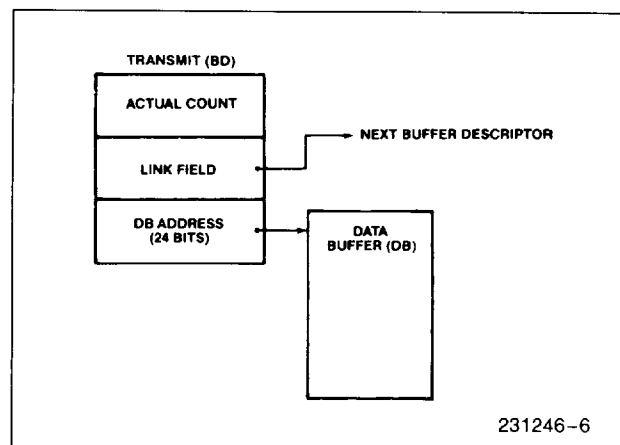
Figure 6. Data Buffer Descriptor and Data Buffer Structure
