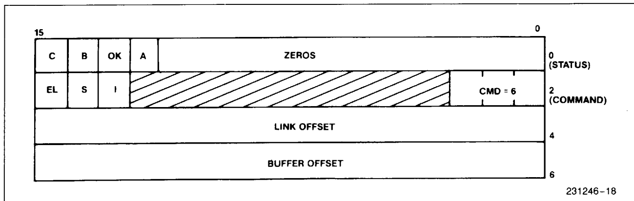
Figure 18. The DUMP Command Block
