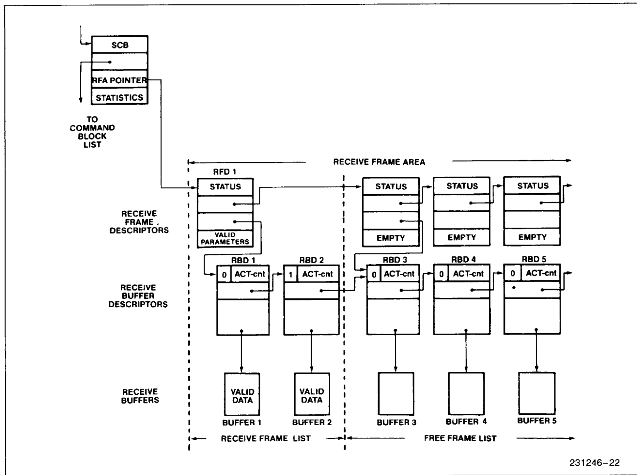
Figure 21. The Receive Frame Area
