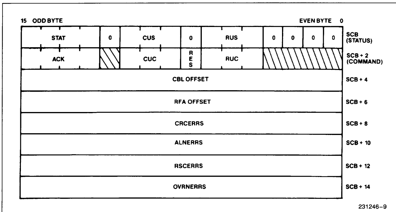
Figure 10. System Control Block (SCB) Format
