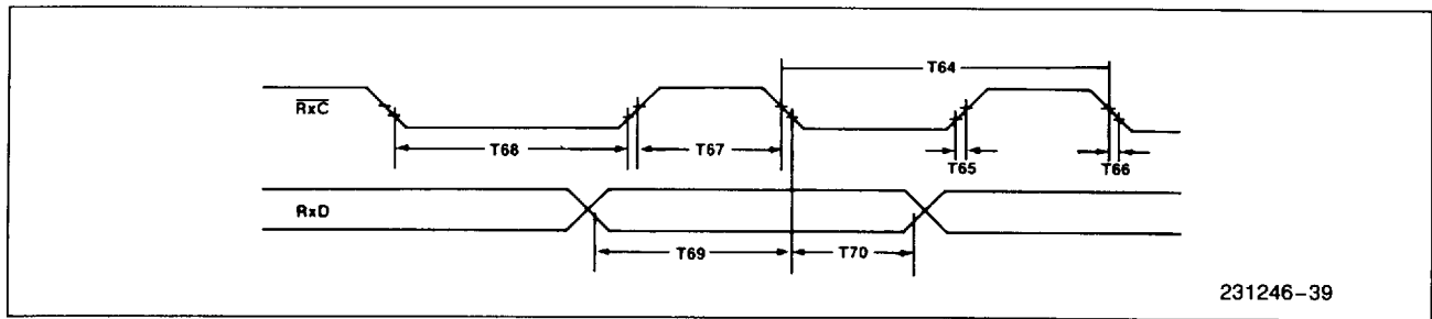
Figure 37. RxD Timing Relative to RxC
