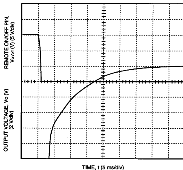
Figure 8. Typical FW150B Start-Up Transient at Room Temperature, 48 V Input, and 12.50 A Output
