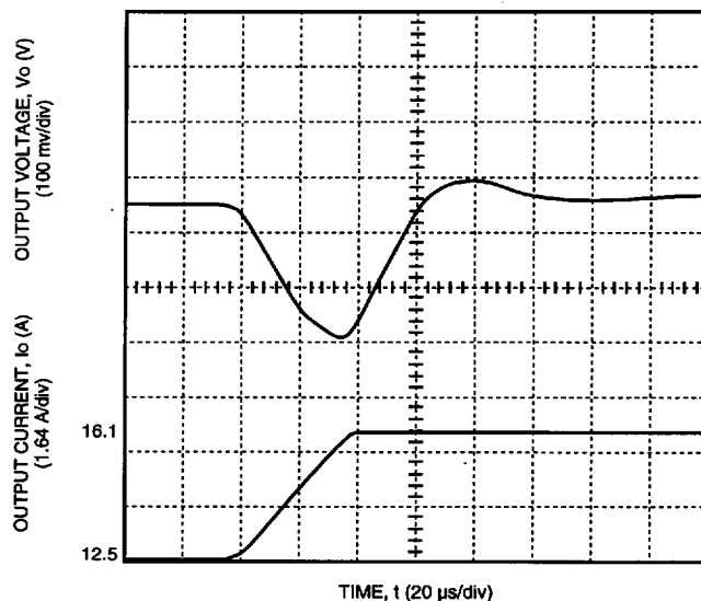
Figure 7. Typical FW150B Transient Response to Step Increase in Load from 50% to 75% of Full Load at Room Temperature and 48 V Input (Waveform Averaged to Eliminate Ripple Component.)
