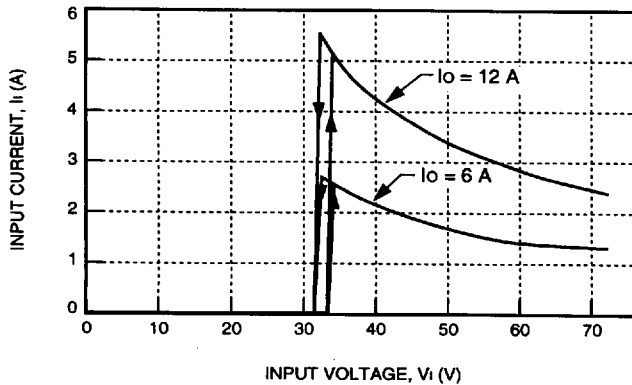
Figure 1. Typical FW150B Input Characteristics at Room Temperature
