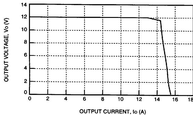
Figure 2. Typical FW150B Output Characteristics at Room Temperature and 48 V Input
