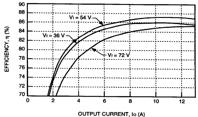
Figure 4. Typical FW150B Efficiency vs. Output Current at Room Temperature
