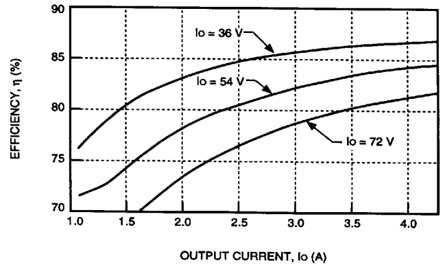
Figure 3. Typical FW050B Efficiency vs. Output Current at Room Temperature
