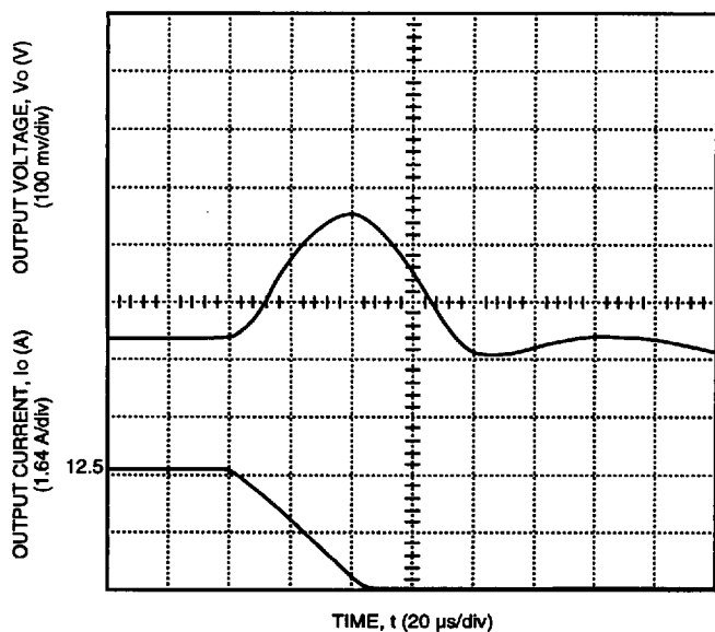
Figure 6. Typical FW150B Transient Response to Step Decrease in Load from 50% to 25% of Full Load at Room Temperature and 48 V Input (Waveform Averaged to Eliminate Ripple Component.)
