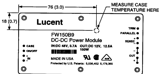
Figure 18. Case Temperature Measurement Location
