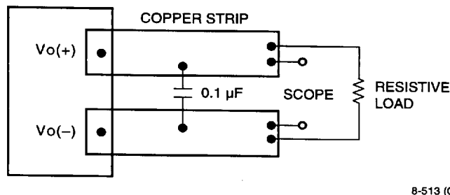
Figure 10. Output Voltage and Efficiency Measurement Test Setup
