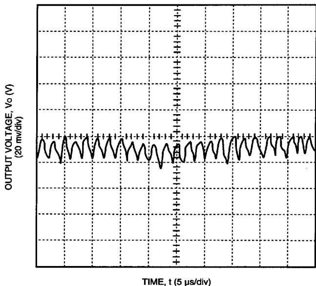
Figure 5. Typical FW150B Output Ripple Voltage at Room Temperature, 48 V Input, and 12.50 A Output
