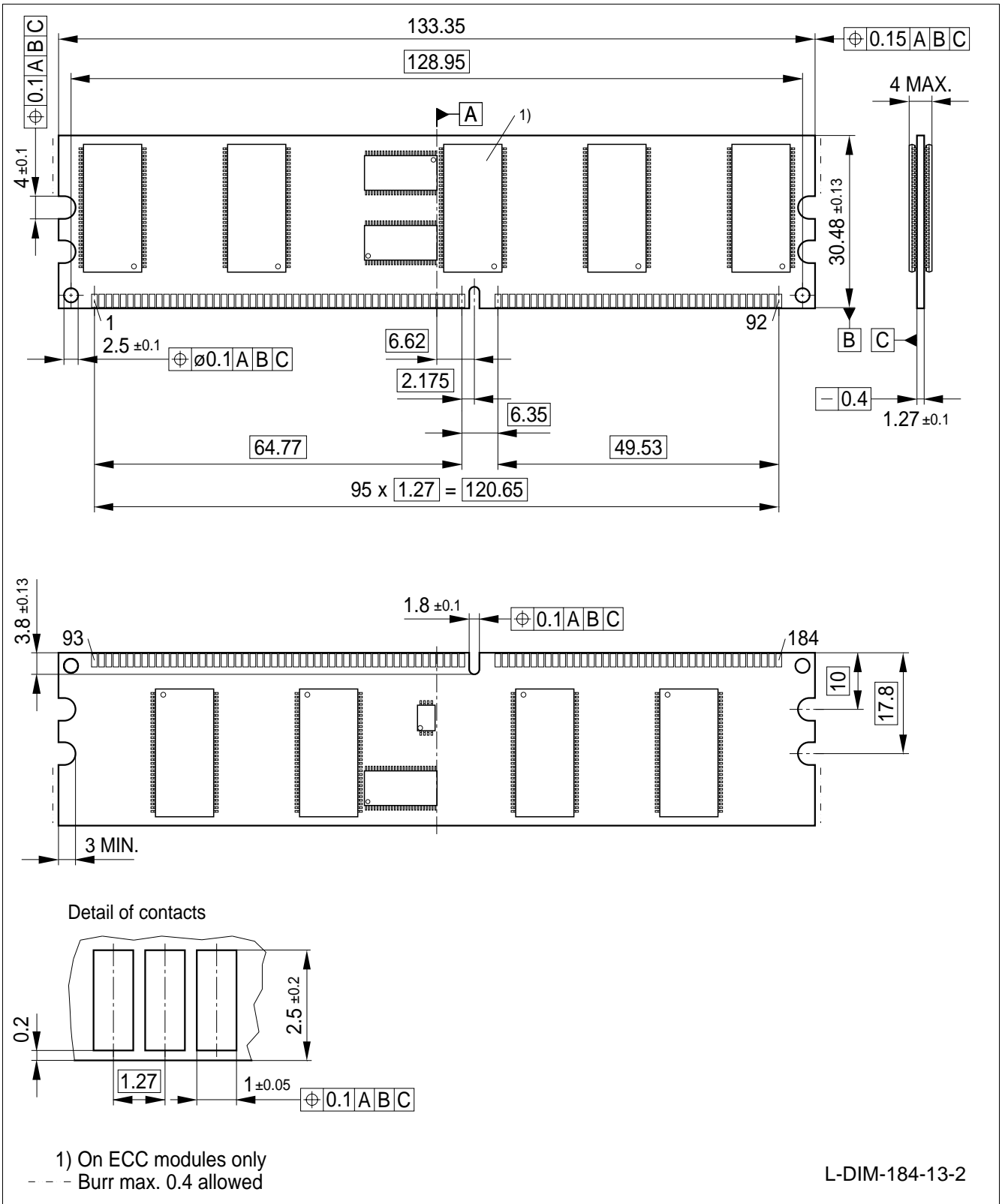
Figure 5 Package Outline: Raw Card L HYS72D16500HR-7-C
