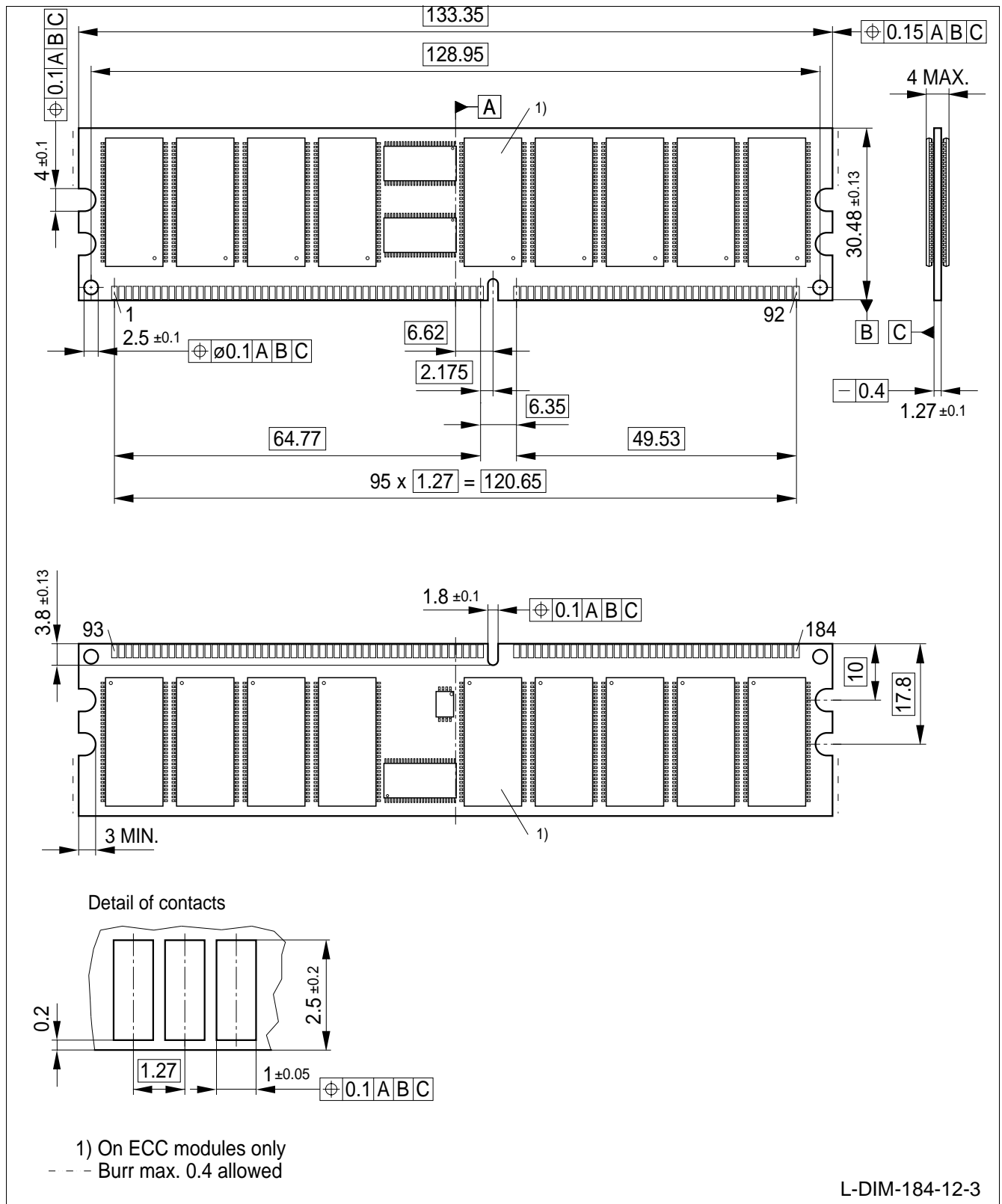
Figure 4 Package Outlines: Raw Card M HYS72D32501HR-7-C
