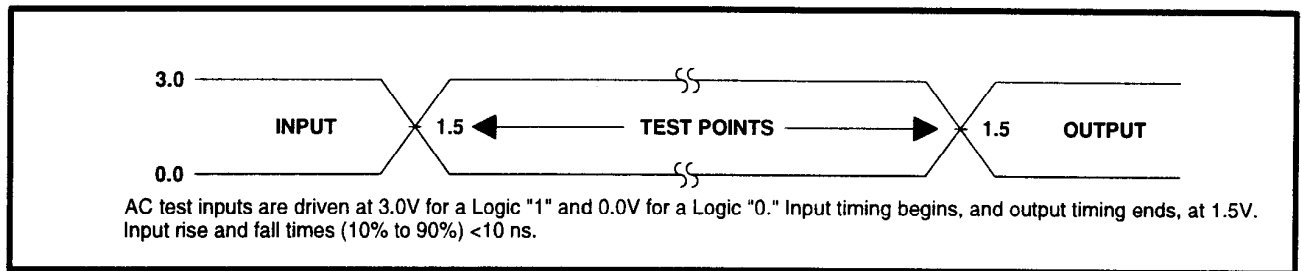
Figure 14. Transient Input/Output Reference Waveform for V_{CC}=5V\pm0.25V (High Speed Testing Configuration)
