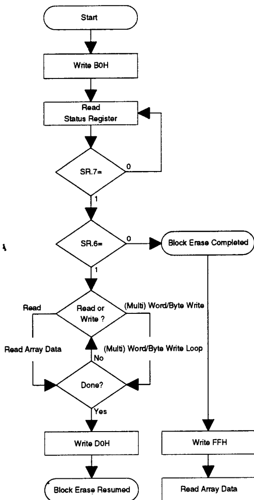
Figure 10. Block Erase Suspend/Resume Flowchart
