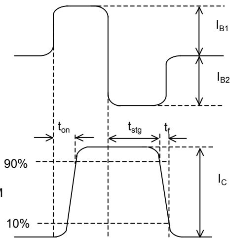
COLLECTOR CURRENT WAVEFORM
