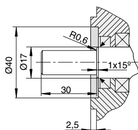
Detail Y:
