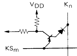
Transistor Switch
