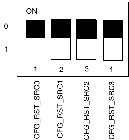
Figure 27. DIP Switch S3
