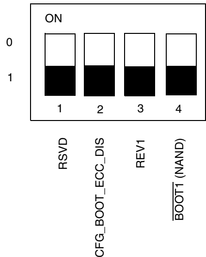
Figure 28. DIP Switch S4
