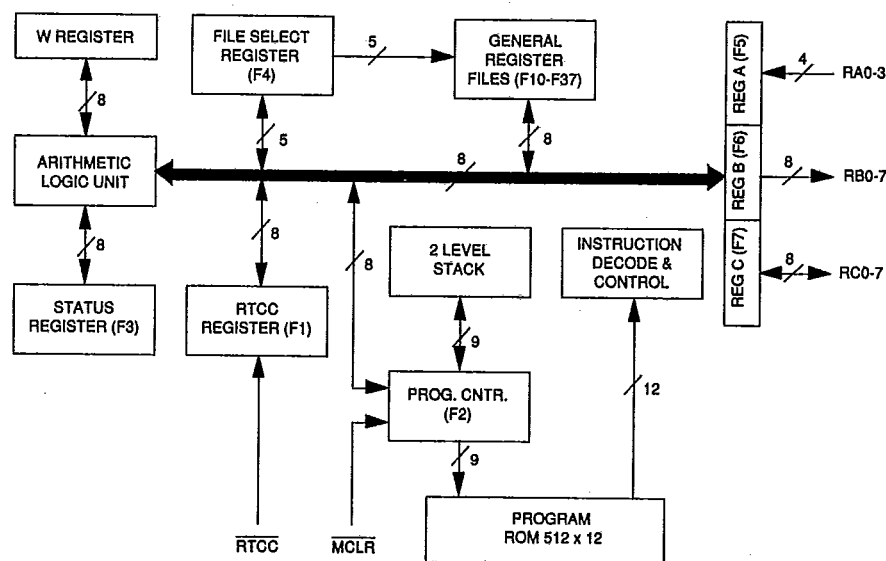
PIC1655 BLOCK DIAGRAM
