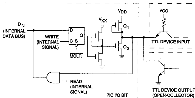
TYPICAL INTERFACE-BIDIRECTIONAL I/O LINE
