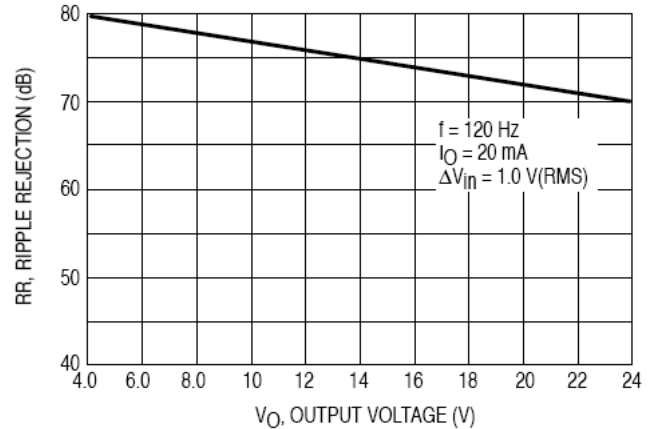
Figure 2. Ripple Rejection as a Function of Output Voltage
