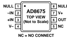
Figure 2. 8-Lead MSOP (RM-8)
