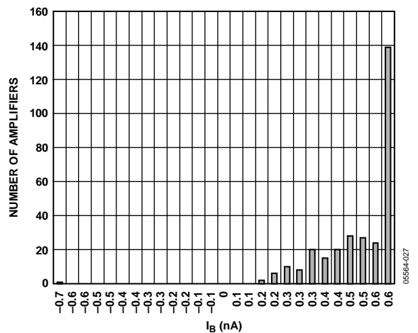
Figure 8. Input Bias Current, V_{SV} = \pm 5\text{ V}
