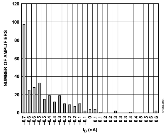
Figure 7. Input Bias Current, V_{SV} = \pm 15\text{ V}
