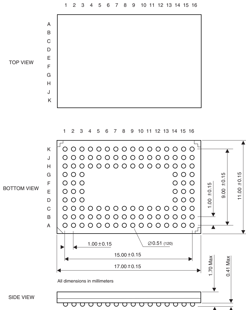
Figure 2. 120-ball BGA Package
