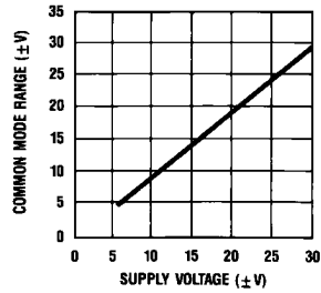
Input Common Mode Range vs Supply Voltage
