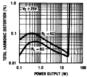
THD vs Power Output
