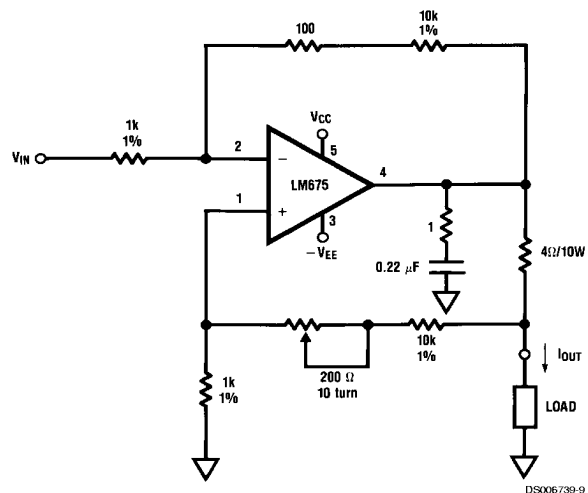
High Current Source/Sink
