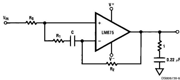
Non-Inverting Unity Gain Operation
