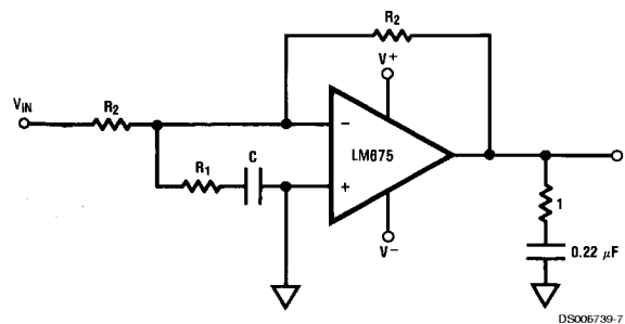
Inverting Unity Gain Operation
