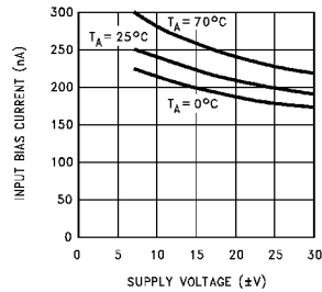
I_B vs Supply Voltage
