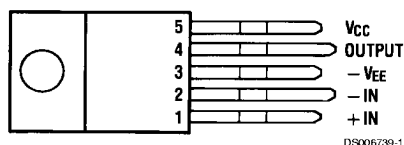
TO-220 Power Package (T)
