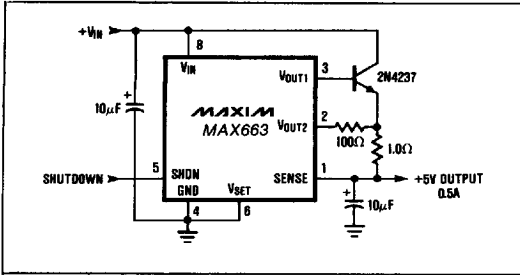
Figure 9. Positive Regulator With Boosted Output, Current Limit, and Low I_O Shutdown
