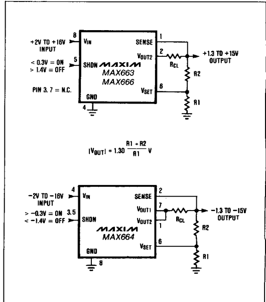
Figure 5. Connections for Adjustable Output
