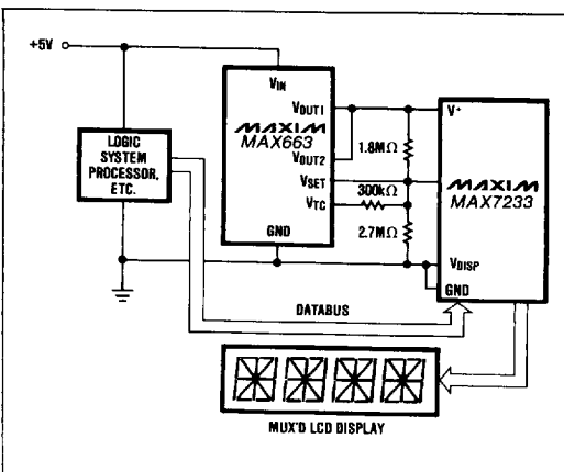
Figure 8. Driving a Multiplexed LCD Display. Consistent operation over more than 40^{\circ}C temperature span, as opposed to about 10^{\circ}C with fixed drive voltage, is allowed by negative temperature coefficient drive voltage to the displays. Based on EPSON LDB-728 Display or equivalent.
