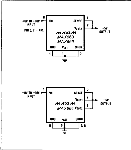
Figure 4. Connections for Fixed 5V Output
