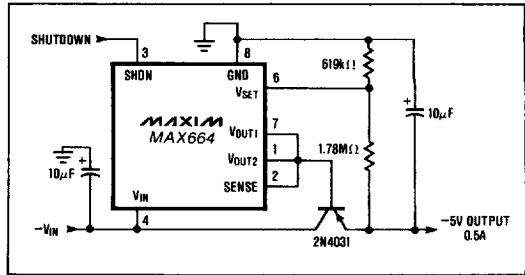
Figure 10. Negative Regulator With Boosted Output and Low I_O Shutdown
