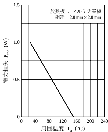
P_{\text{tot}} - T_a
