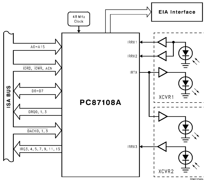
FIGURE 2. Basic Configuration
