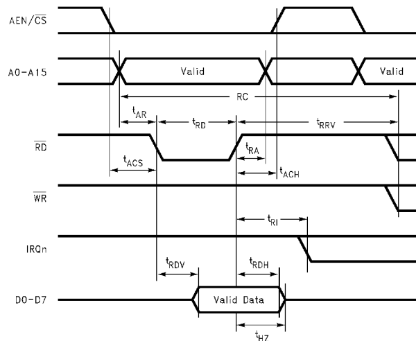
FIGURE 42. CPU Read Timing
