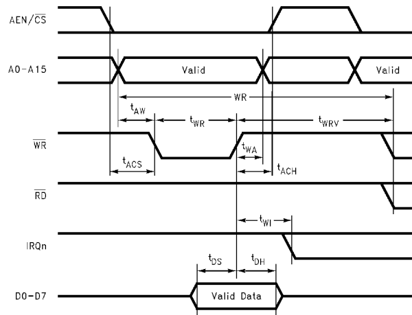
FIGURE 43. CPU Write Timing
