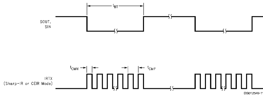
FIGURE 45. UART, Sharp-IR and Consumer-IR Timing
