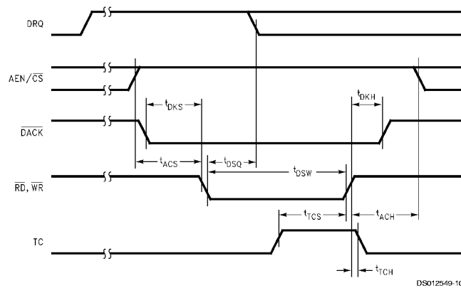
FIGURE 44. DMA Access Timing
