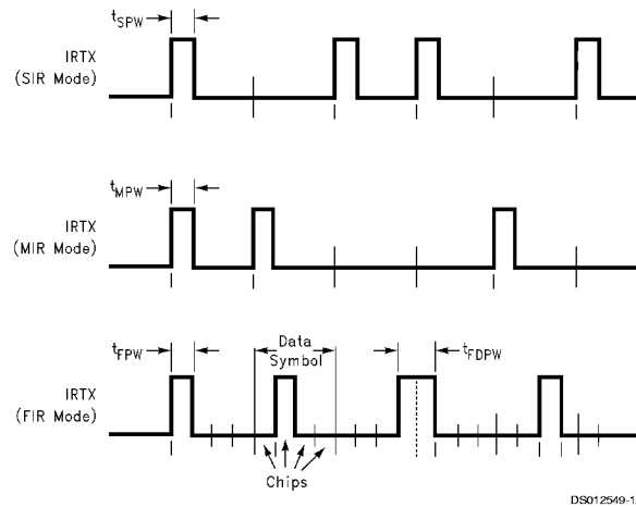
FIGURE 46. SIR, MIR and FIR Timing
