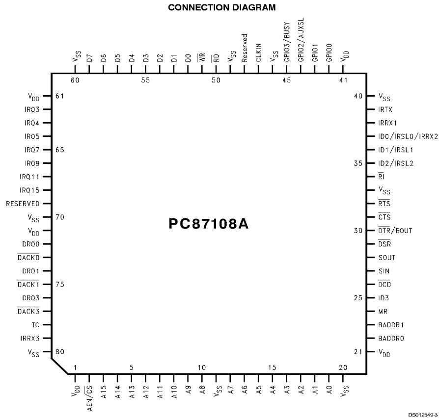
Top View FIGURE 1. 80-Pin PQFP or TQFP Package
