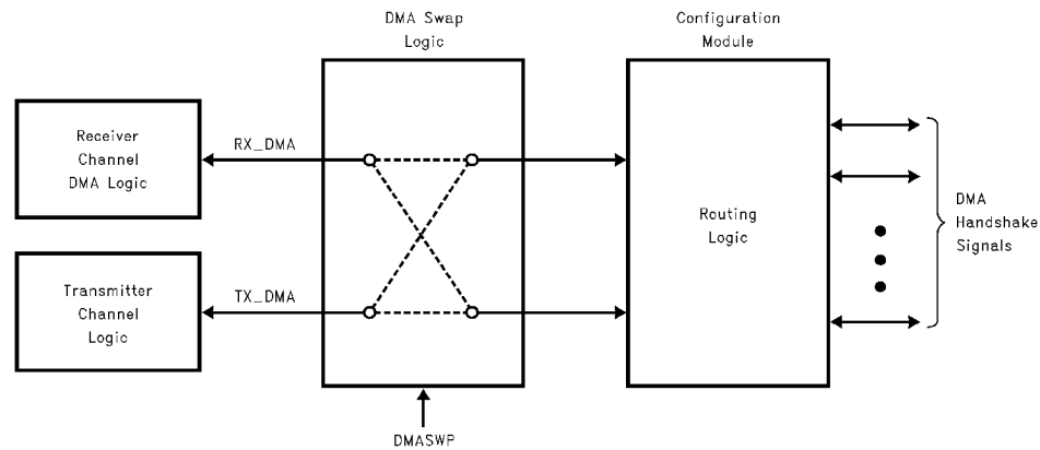
FIGURE 16. DMA Control Signals Routing
