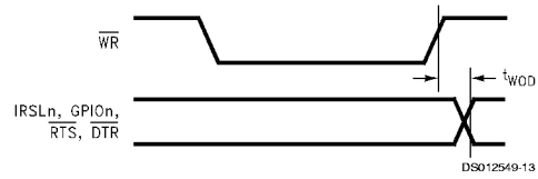
FIGURE 47. GPIOn and IRSLn Write Timing
