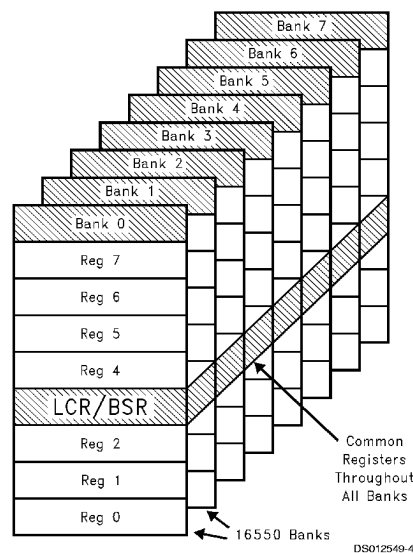
FIGURE 4. Register Bank Architecture
