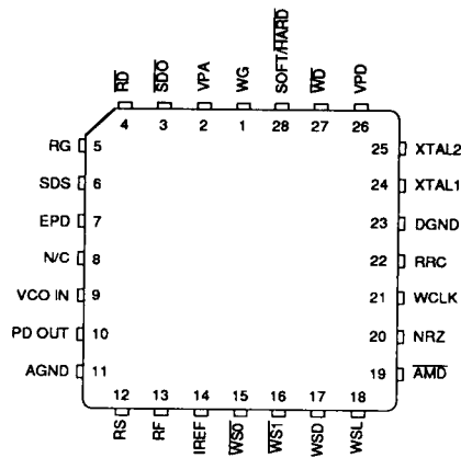
28-Pin PLCC
