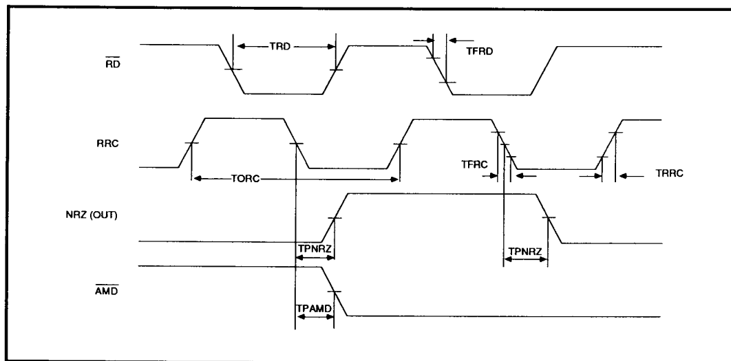
FIGURE 9: Read Timing
