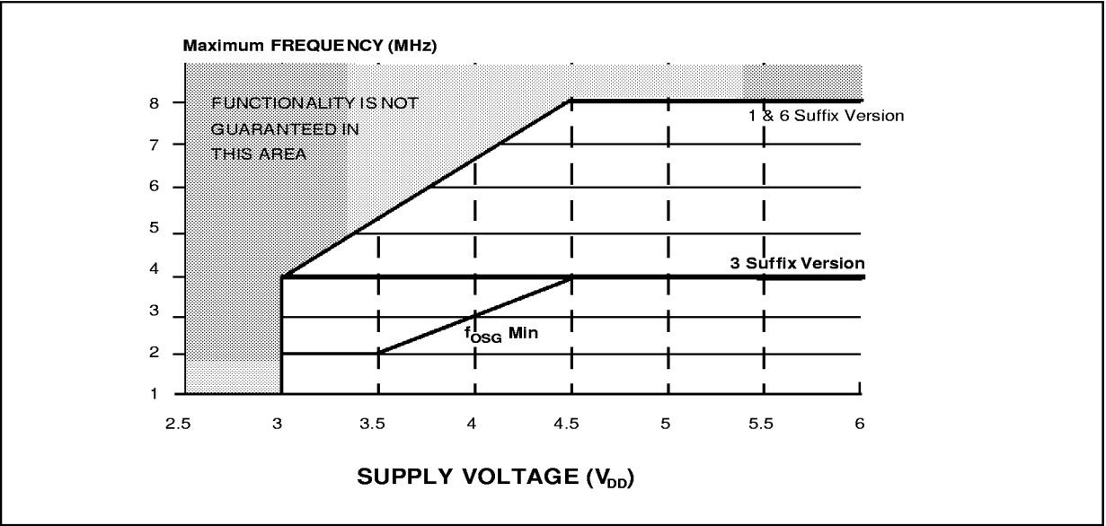
Figure 36. Maximum Operating FREQUENCY (Fmax) Versus SUPPLY VOLTAGE ( V_{DD} )
