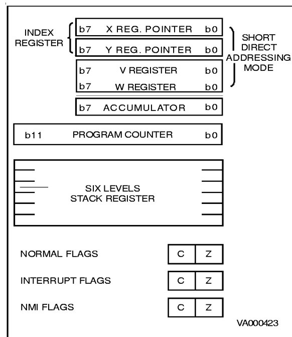
Figure 7 ST6 CPU Programming Mode
