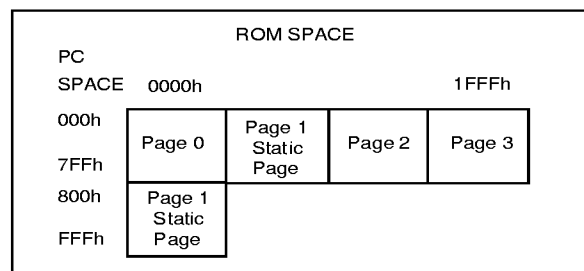
Figure 3. 8Kbytes Program Space Addressing
