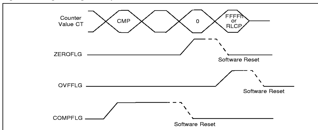
Figure 24. Flags Setting in Compare and Reload Functions
