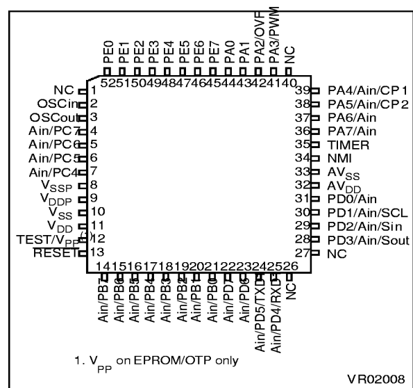
Figure 2. ST62T35B/E35B Pin Configuration
