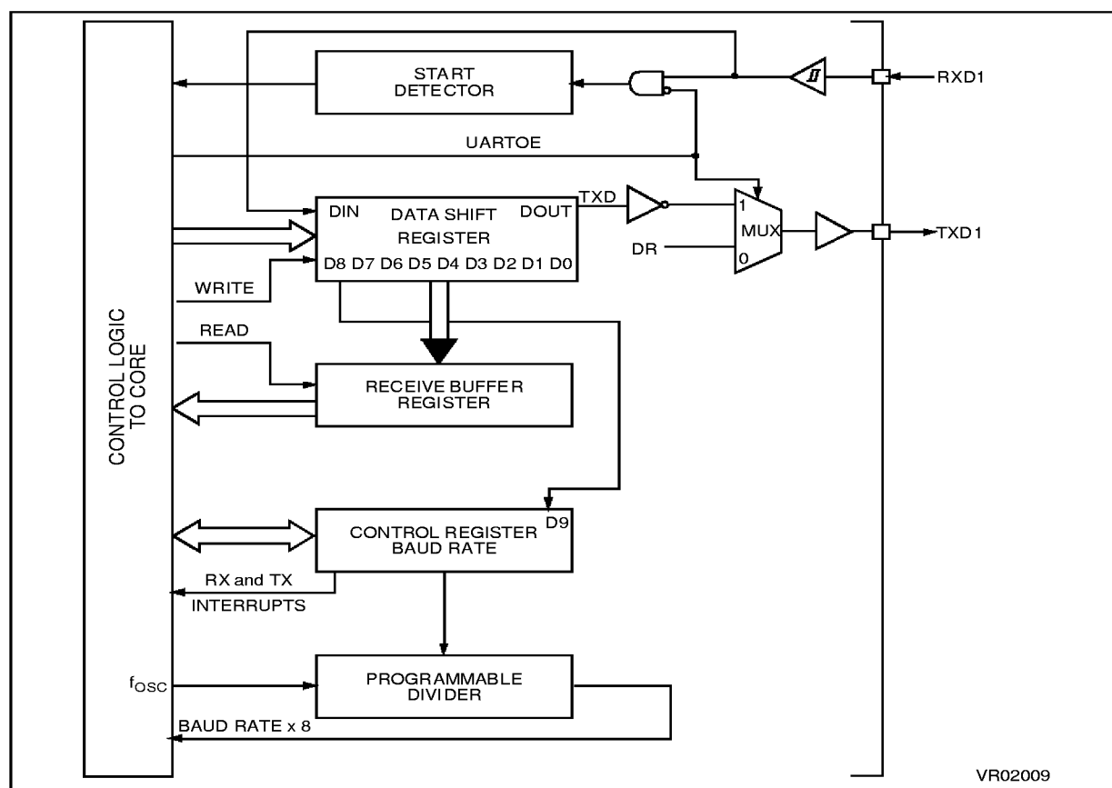
Figure 31. UART Block Diagram
