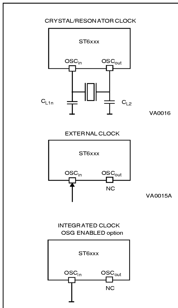
Figure 8. Oscillator Configurations
