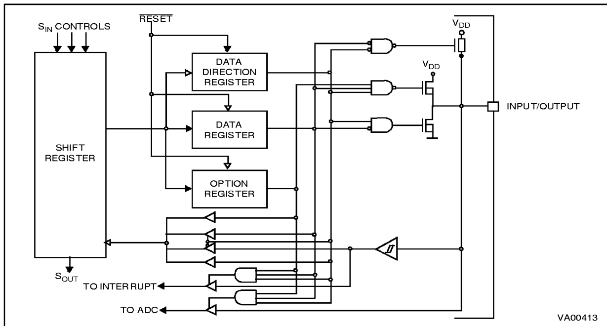
Figure 18. I/O Port Block Diagram
