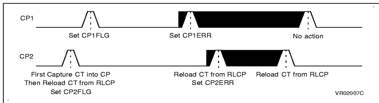
Figure 27. . CP2 Triggered Restart Mode with CP2 Event Detection
