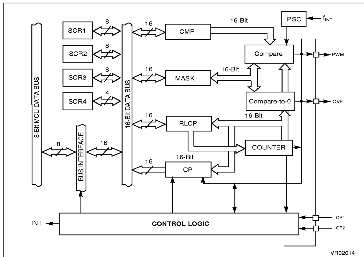
Figure 23. . ARTIMER16 Block Diagram
