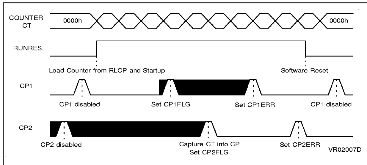
Figure 28. . Software Triggered Restart Mode with CP2 Event Detection
