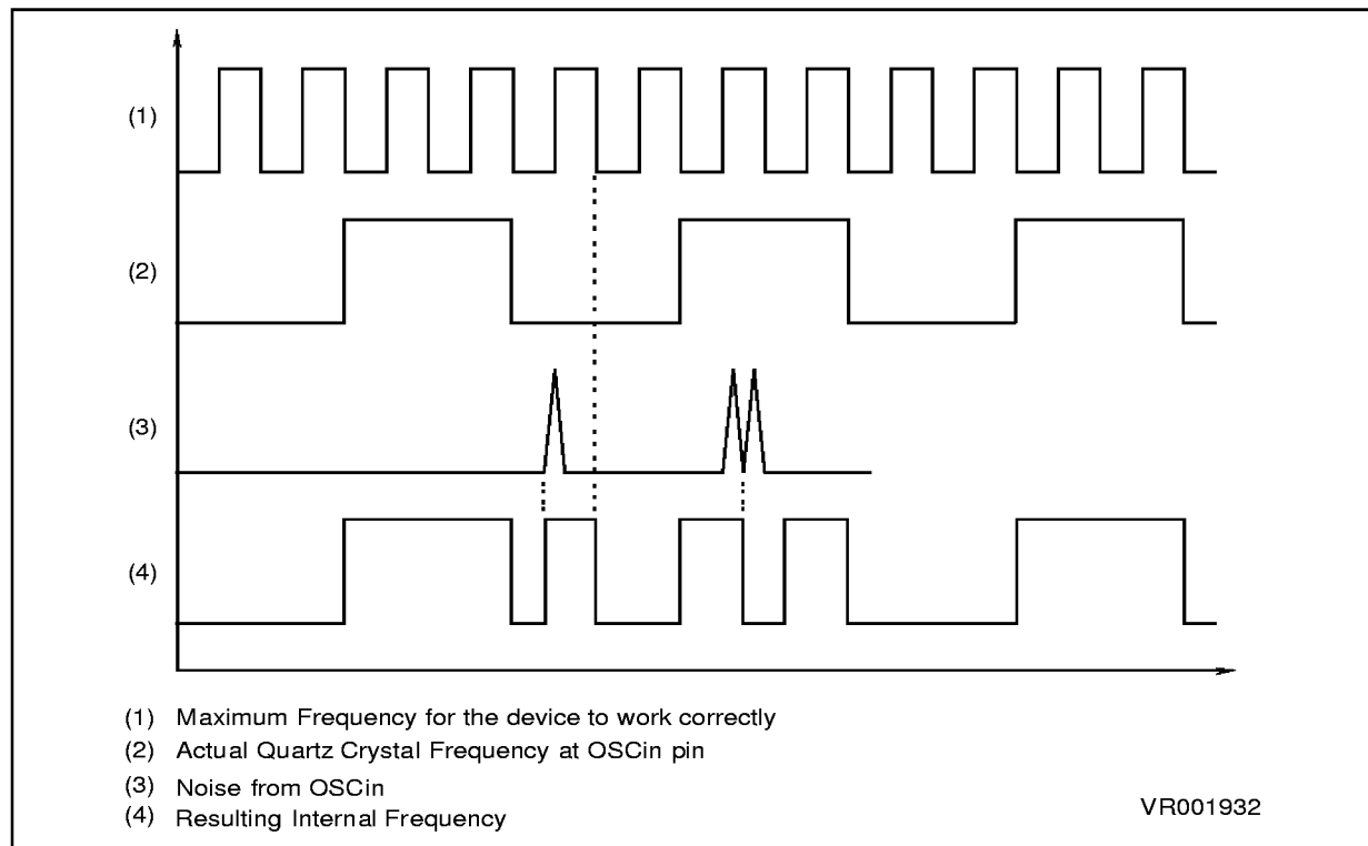
Figure 10. OSG Emergency Oscillator Principle
