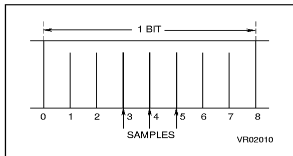
Figure 32. Data Sampling Points
