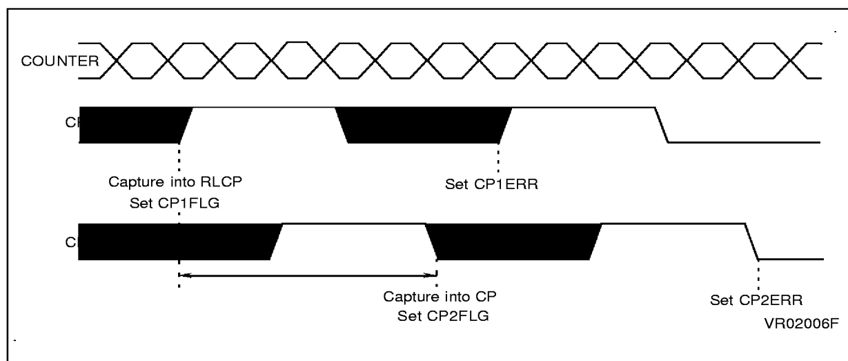
Figure 29. . Positive CP1 - to negative CP2-Edge Measurement (CP1POL = 1, CP2POL = 0)
