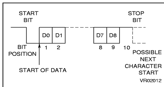
Figure 33. Character Format
