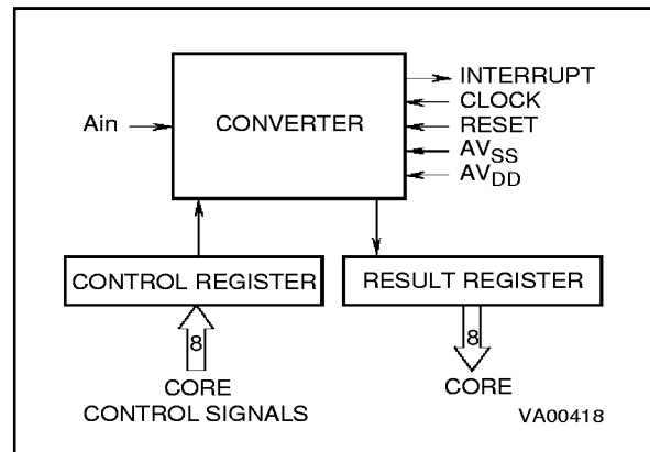
Figure 30. ADC Block Diagram
