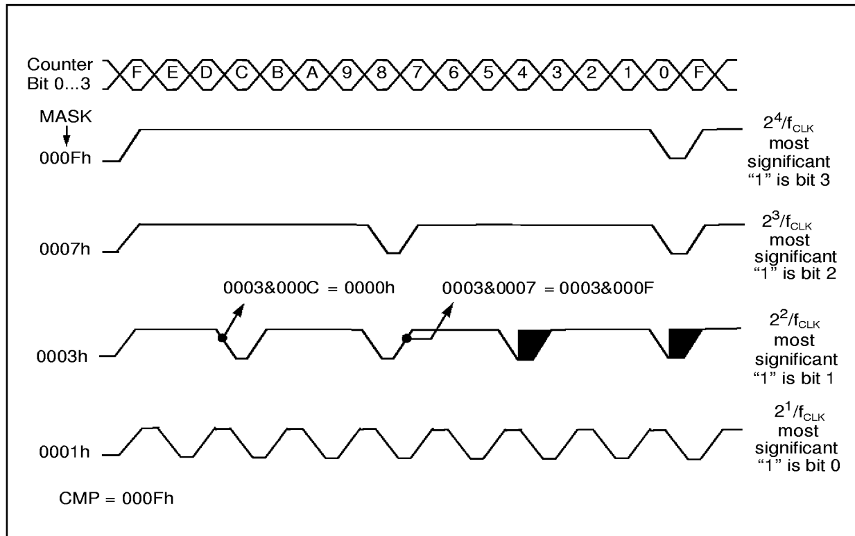
Figure 25. . Mask Impact on the Compare Functions in PWM mode (PWMD=0, PWMPOL=1)
