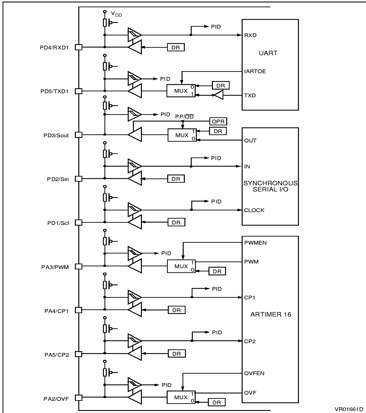
Figure 20. Peripheral Interface Configuration of SPI, UART and AR Timer16
