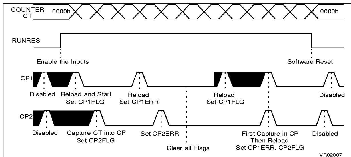
Figure 26. . CP1 Triggered Restart Mode with CP2 Event Detection
