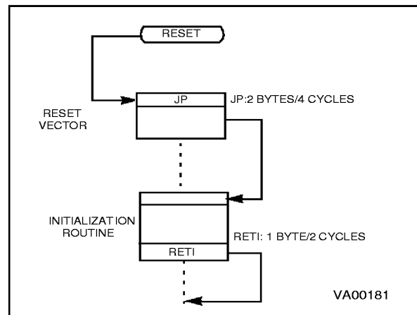
Figure 14. Reset and Interrupt Processing
