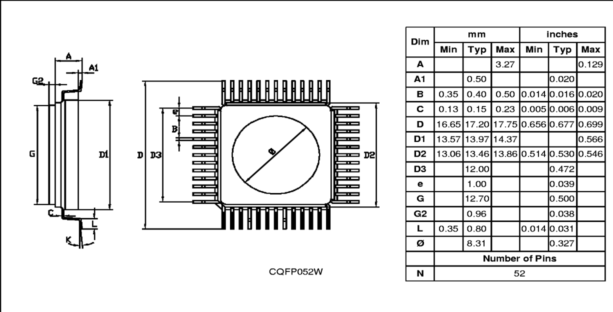
Figure 38. 52-Pin Ceramic Quad Flat Package with Window
