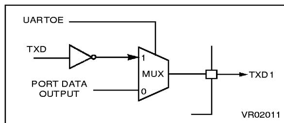
Figure 34. .UART Data Output
