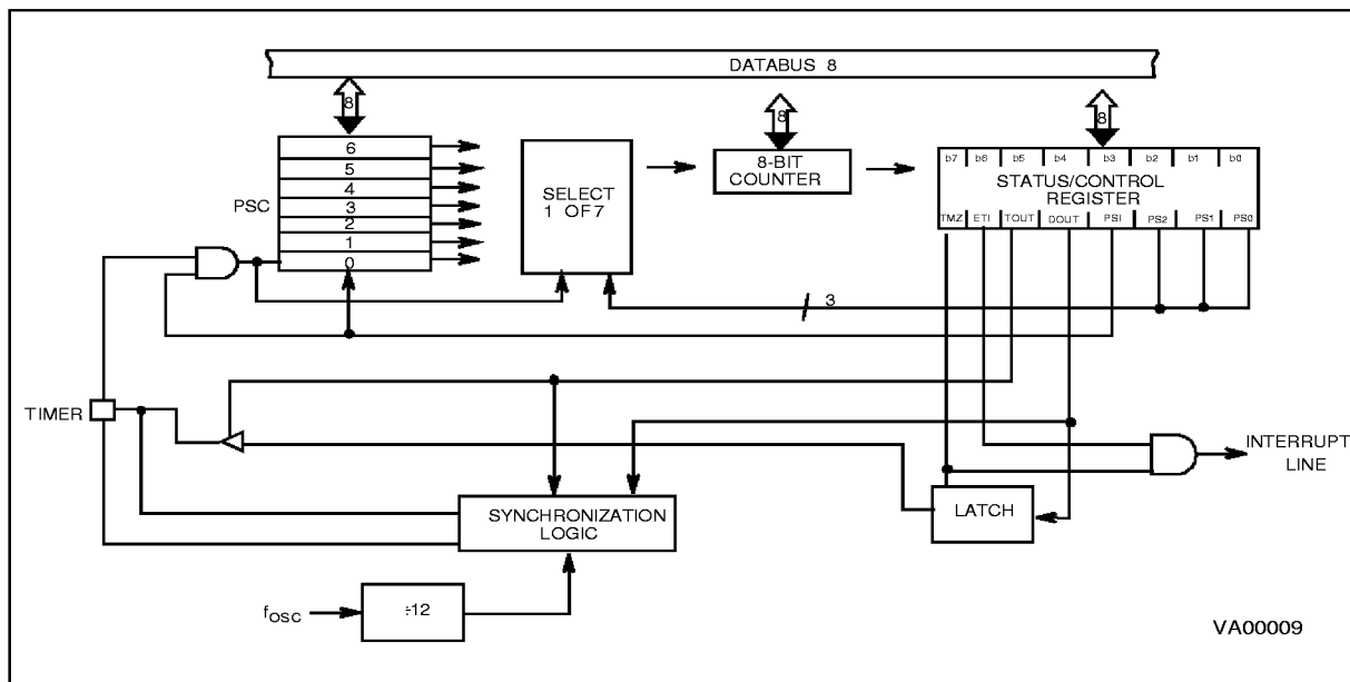
Figure 21. Timer Block Diagram
