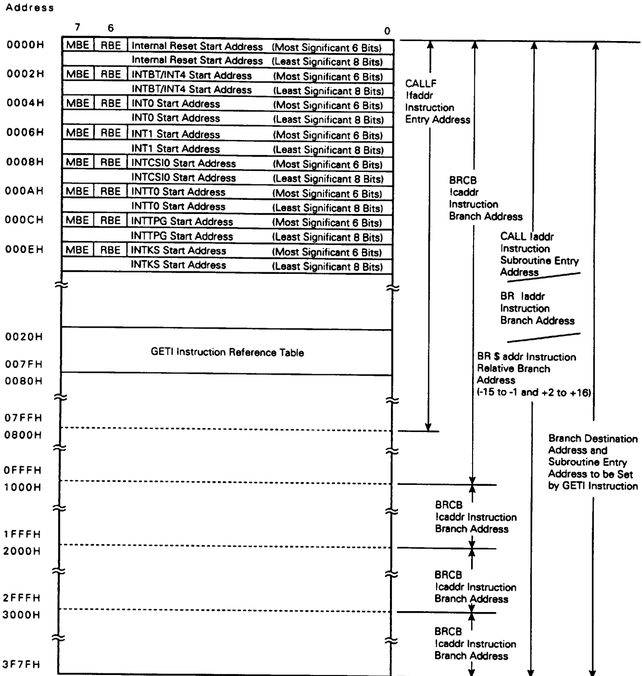
Fig. 4-1 Program Memory Map
