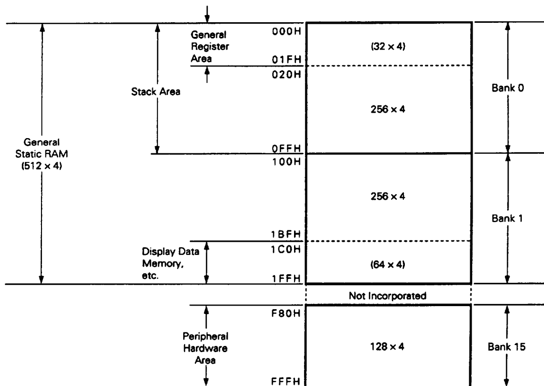
Fig. 4-2 Data Memory Map
