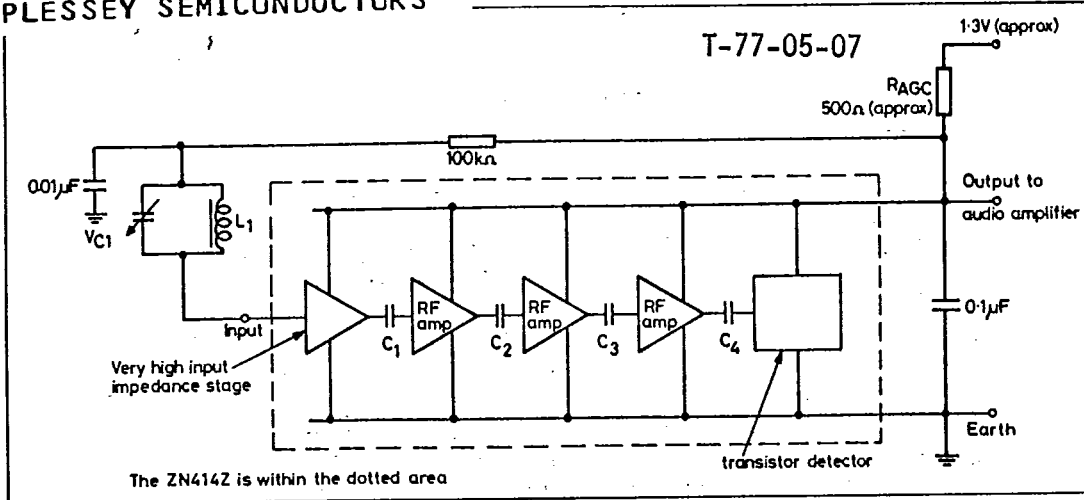
ZN414Z System Diagram
