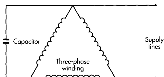
Connection diagram
