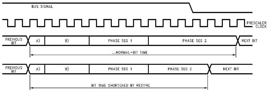
FIGURE 31. Resynchronization 2
