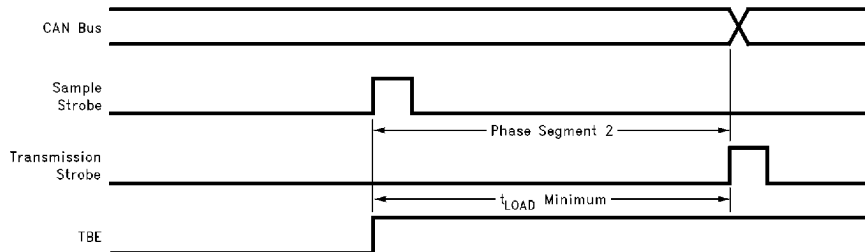
FIGURE 17. TBE Timing
