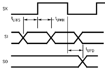
FIGURE 3. MICROWIRE/PLUS Timing Diagram
