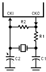
FIGURE 7. Crystal Oscillator Diagram
