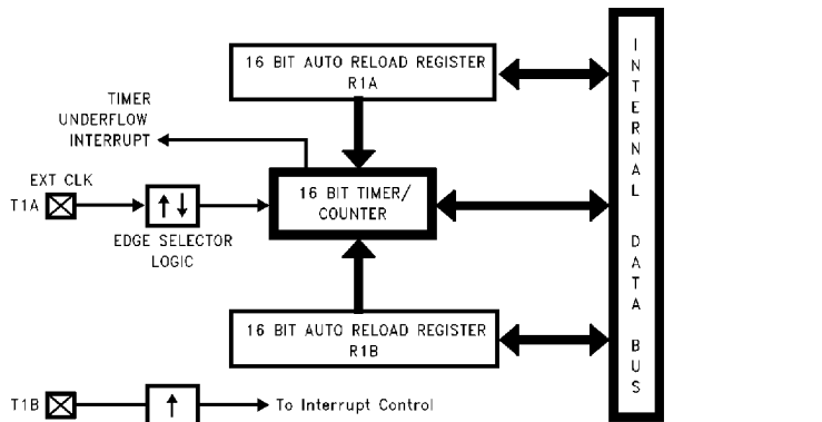
FIGURE 10. Timer 1 in External Event Counter Mode
