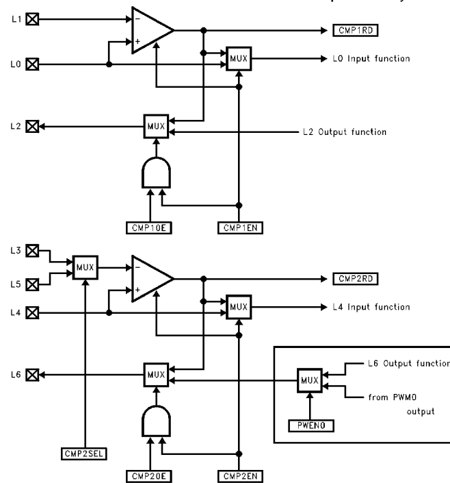
FIGURE 32. Comparator Block
