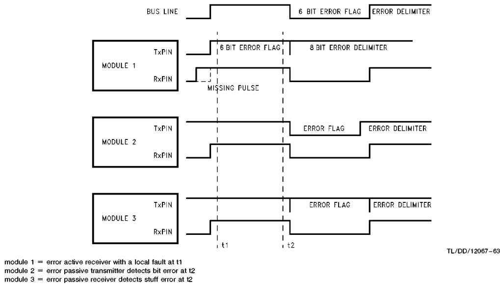
FIGURE 26. Error Frame—Error Passive Transmitter
