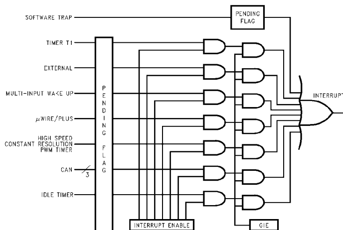
FIGURE 17. Interrupt Block Diagram
