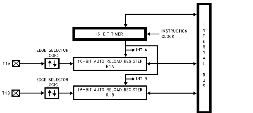
FIGURE 11. Timer 1 in Input Capture Mode
