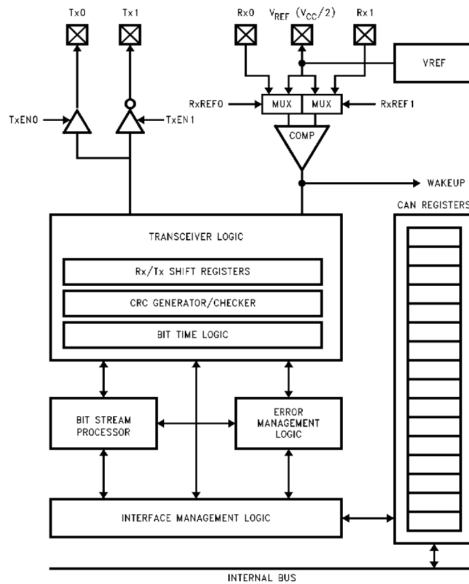
FIGURE 15. CAN Interface Block Diagram
