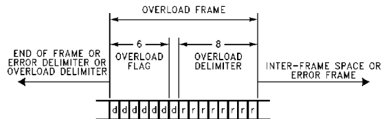
FIGURE 21. CAN Control Frames
