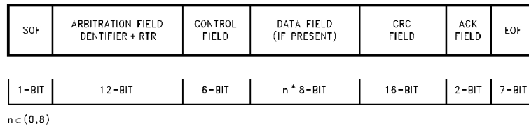
FIGURE 22. CAN Frame Format
