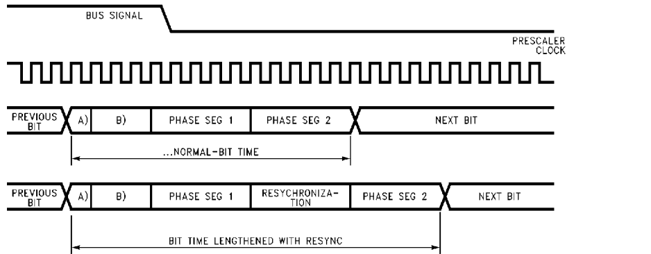
FIGURE 30. Resynchronization 1
