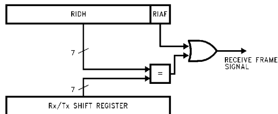
FIGURE 18. Acceptance Filter Block-Diagram
