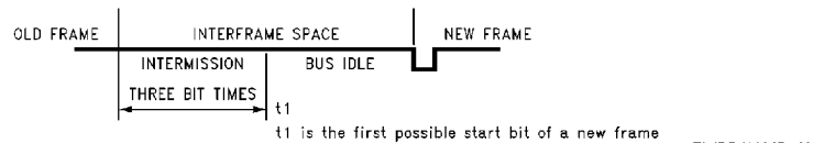
FIGURE 23. Interframe Space for Nodes Which Are Not Error Passive or Have Been Receiver for the Last Frame
