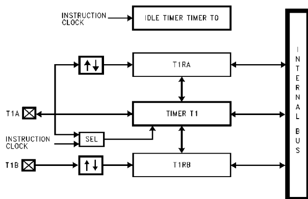
FIGURE 8. Timers T1 and T0
