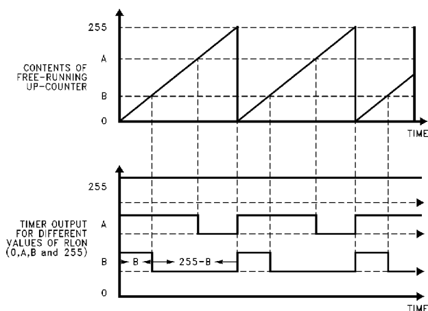
FIGURE 14. PWM Mode Operation
