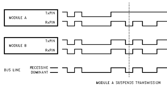
FIGURE 19. CAN Message Arbitration
