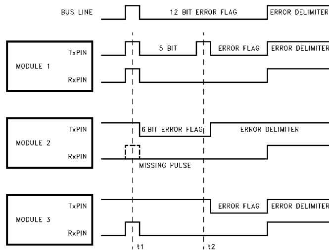
FIGURE 25. Error Frame—Error Active Transmitter
