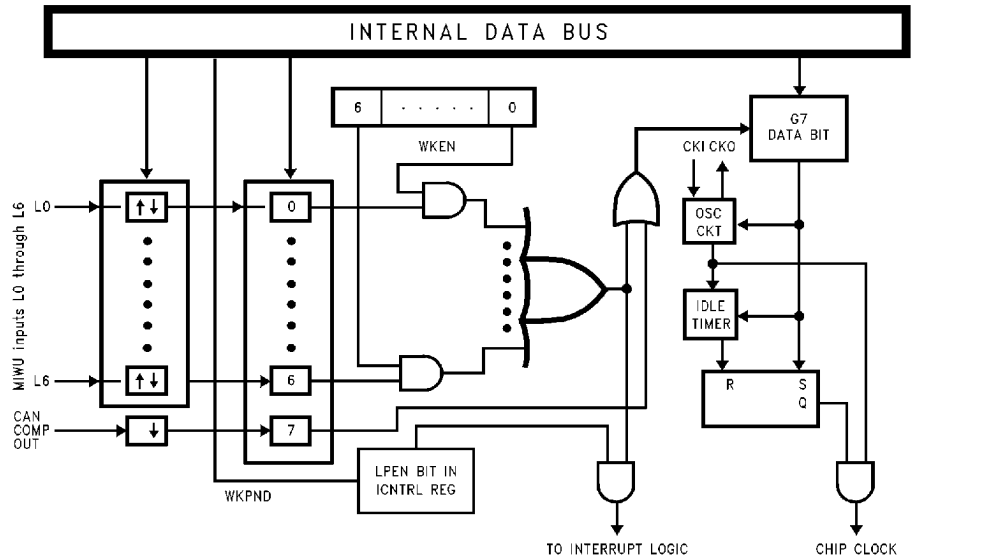
FIGURE 16. Multi-Input Wake Up Logic
