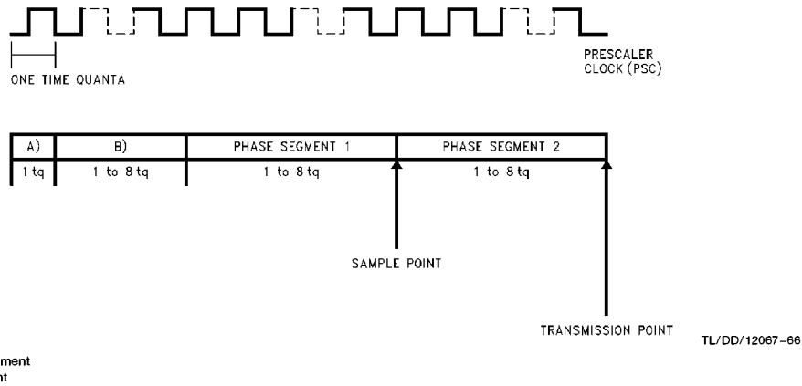
FIGURE 29. Bit Timing
