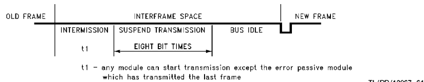
FIGURE 24. Interframe Space for Nodes Which Are Error Passive and Have Been Transmitter for the Last Frame
