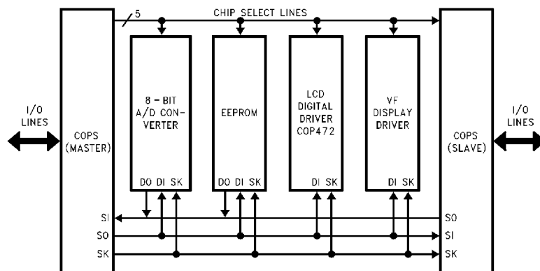
FIGURE 34. MICROWIRE/PLUS Application
