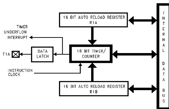
FIGURE 9. Timer 1 in PWM MODE
