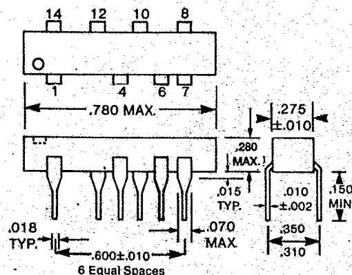
STANDARD DIP-MOUNT
