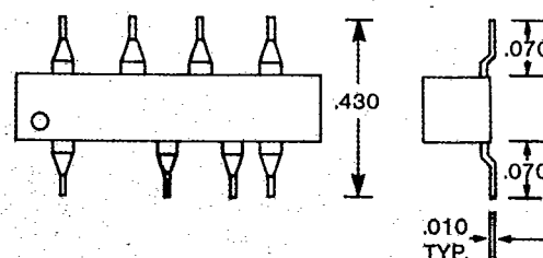
TYPE "A" SURFACE-MOUNT
