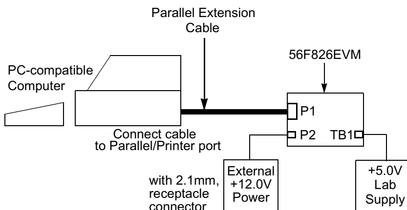
Figure 1-3. Connecting the 56F826EVM Cables
