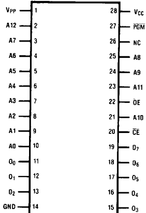
NMC27C64Q/N Dual-In-Line Package
