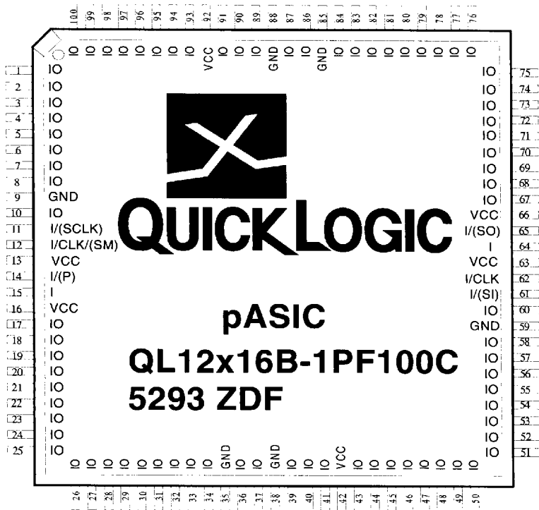
Pinout Diagram 100-pin VQFP/ 100-pin TQFP
