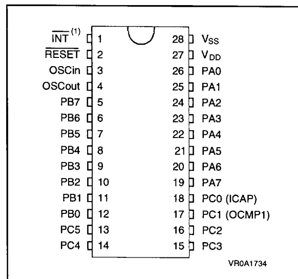
Figure 1. Pin Description
