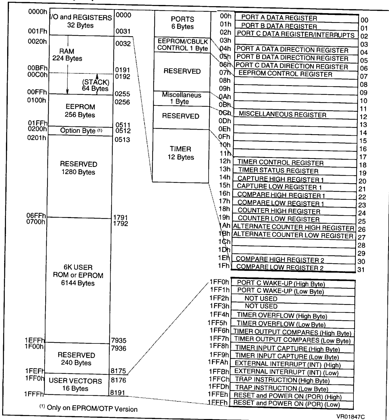
Figure 3. Memory Map
