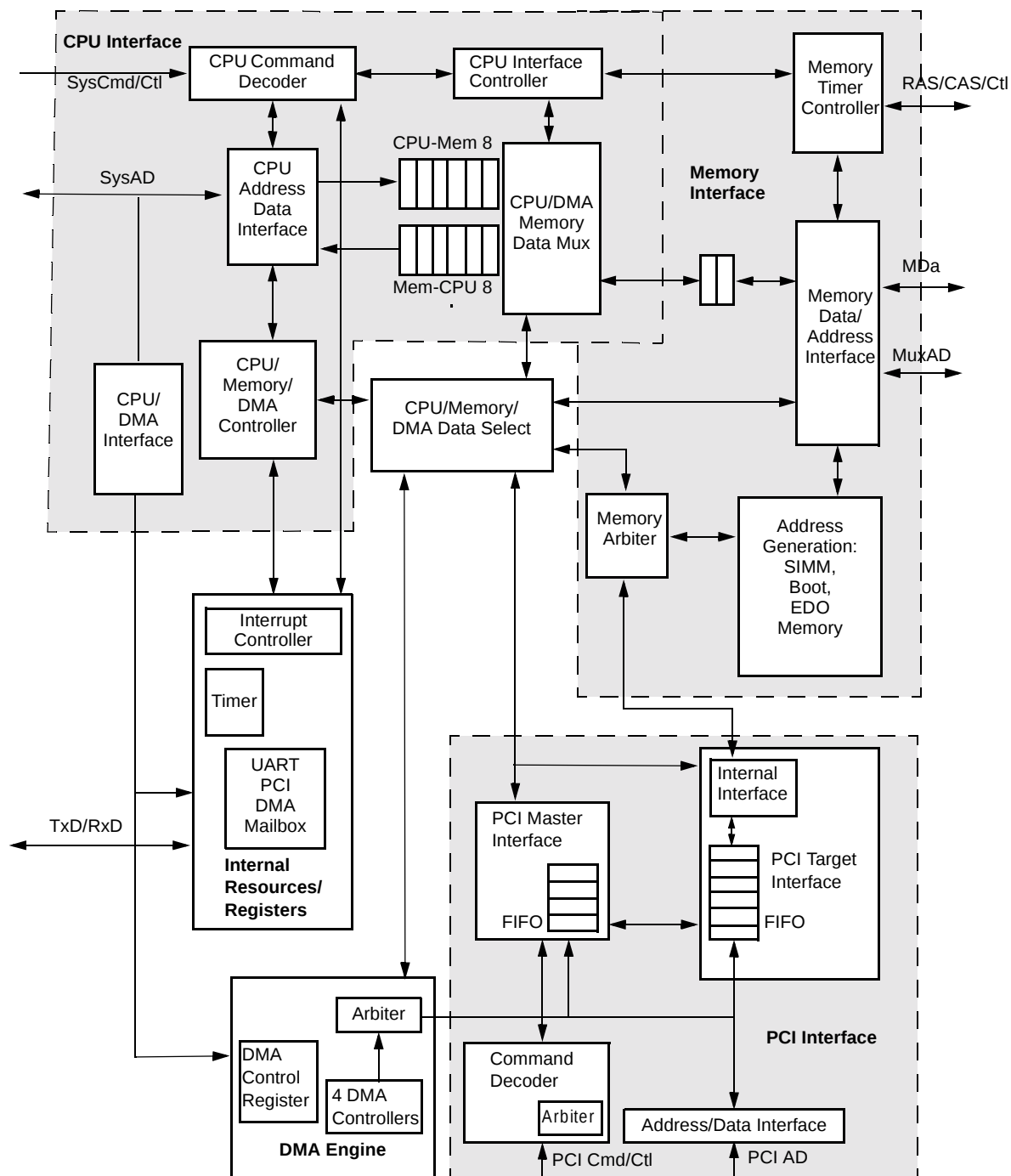
Figure 3. Block Diagram
