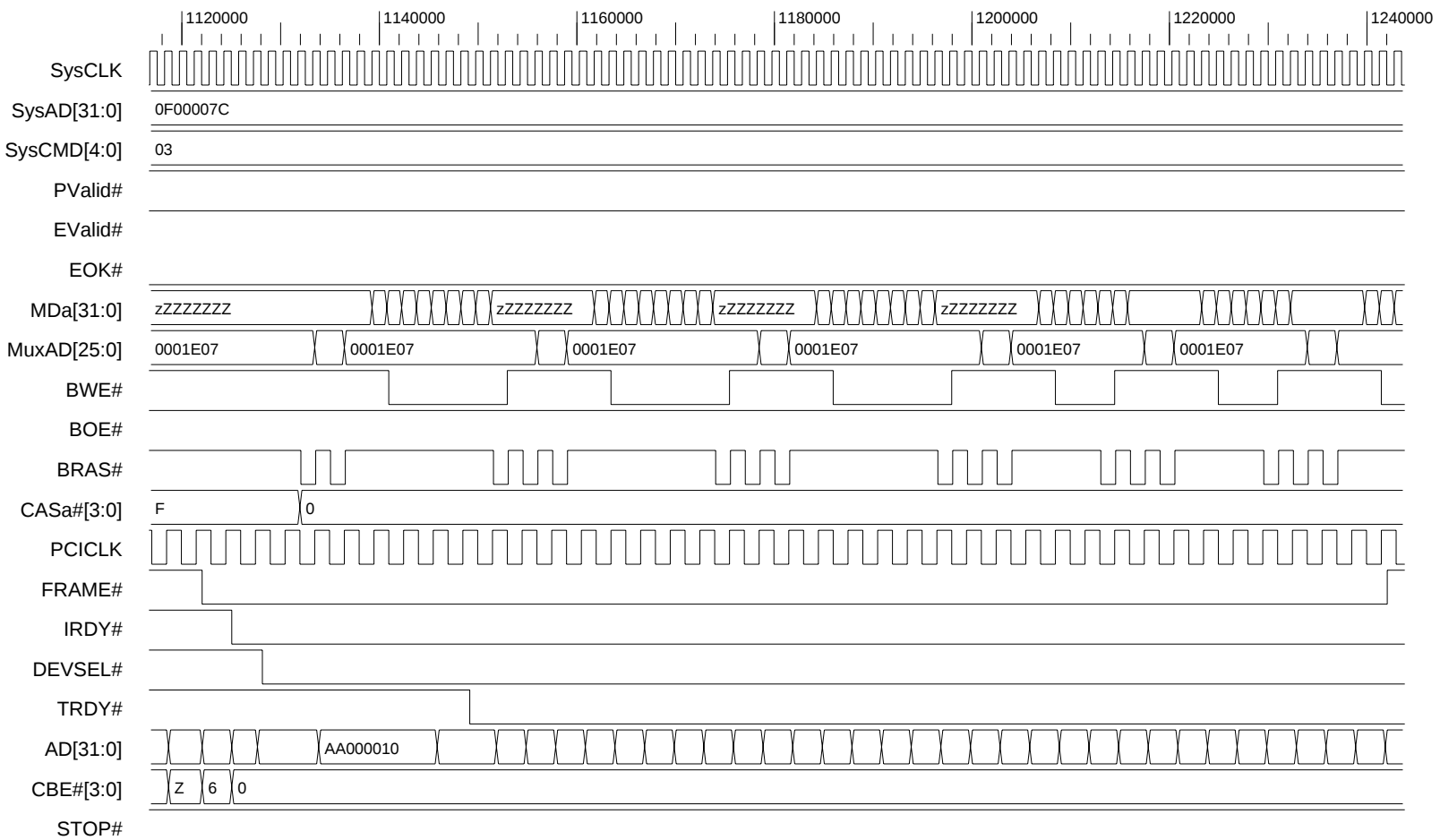
Figure 47. PCI Burst Read: 32 Words
