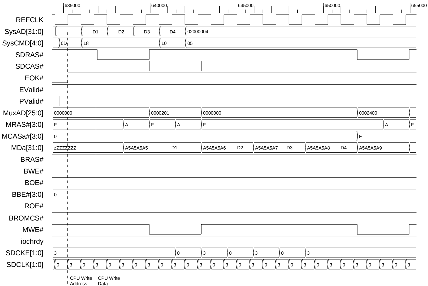
Figure 24. CPU Quad Write to SDRAM SIMM
