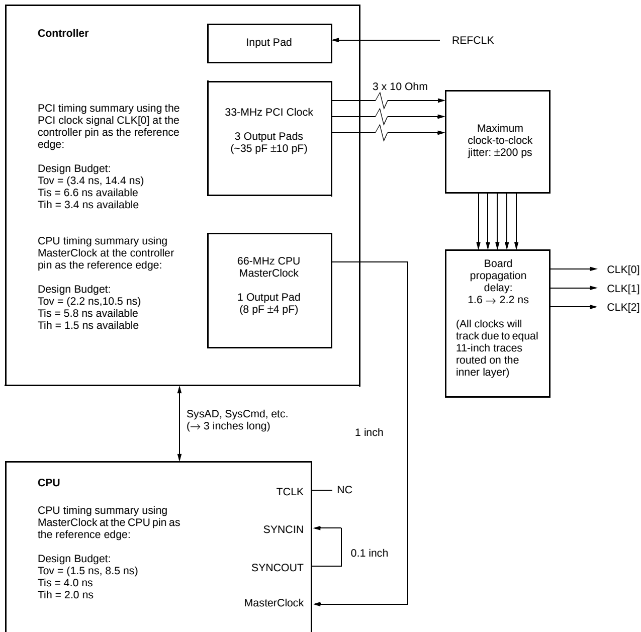
Figure 11. Clock Connections
