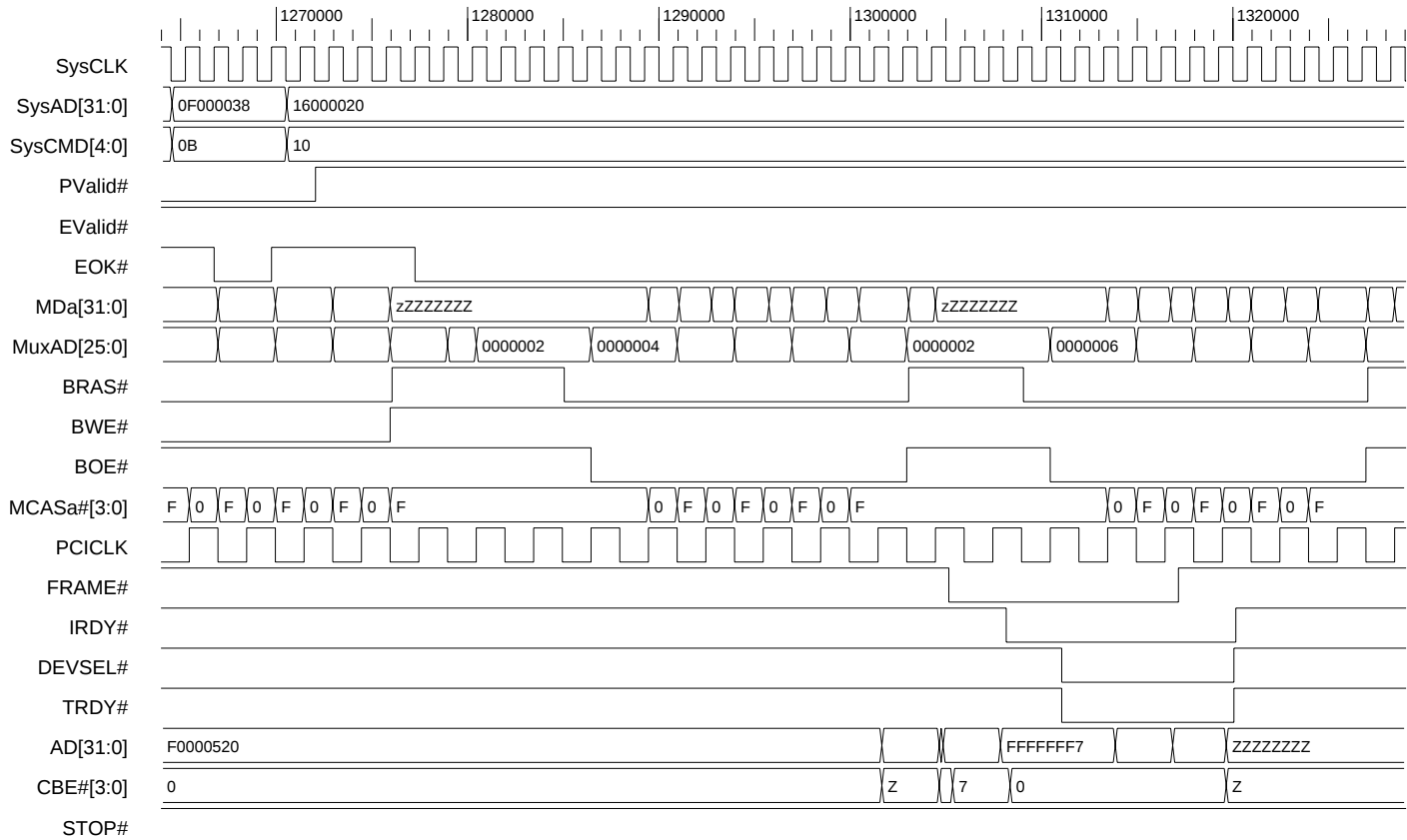
Figure 38. DMA Transfer
