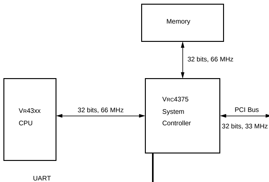
Figure 1. System Connection
