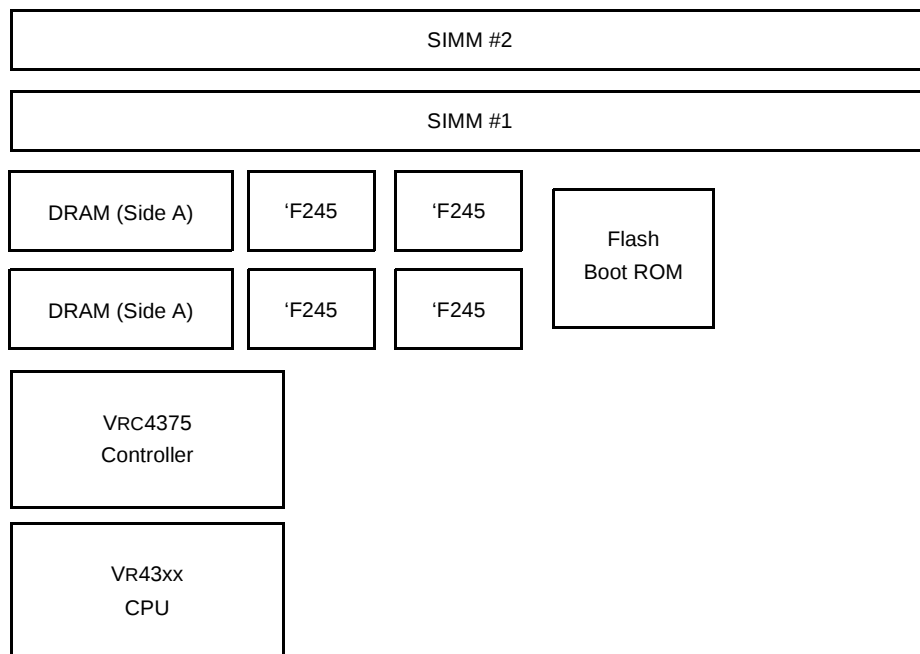
Figure 5. Memory Placement
