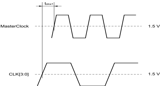
Figure 63. CLK[3:0] versus MasterClock Output Skew at Controller Pins
