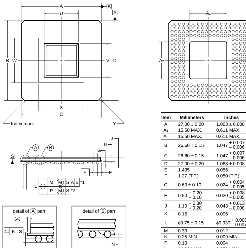
Figure 67. Package Drawing
