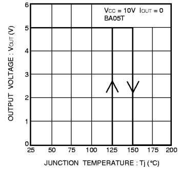
Fig. 8 Thermal cutoff circuit characteristics
