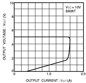
Fig. 9 Current limit characteristics
