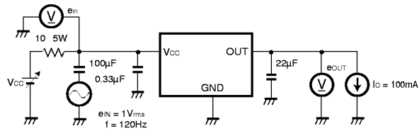
Fig. 2 Measurement circuit for ripple rejection ratio
