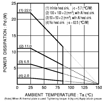
Fig. 6 Ta - power dissipation characteristics (TO220FP)
