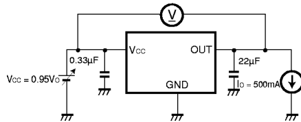
Fig. 3 Measurement circuit for minimum I/O voltage differential
