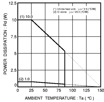
Fig. 7 Ta - power dissipation characteristics (TO 252-3)
