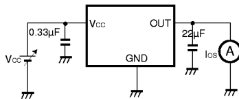
Fig. 5 Measurement circuit for output short-circuit current
