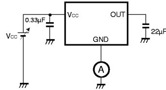
Fig. 4 Measurement circuit for bias current
