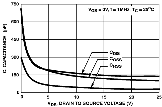
FIGURE 9. TYPICAL CAPACITANCE vs VOLTAGE
