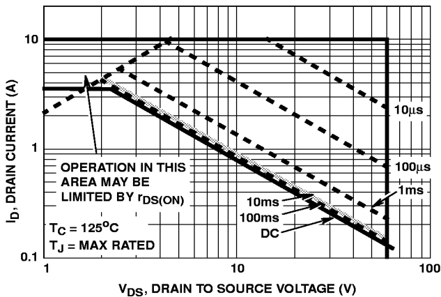
FIGURE 1C. 125^\circ\text{C} SAFE-OPERATING AREA CURVE
