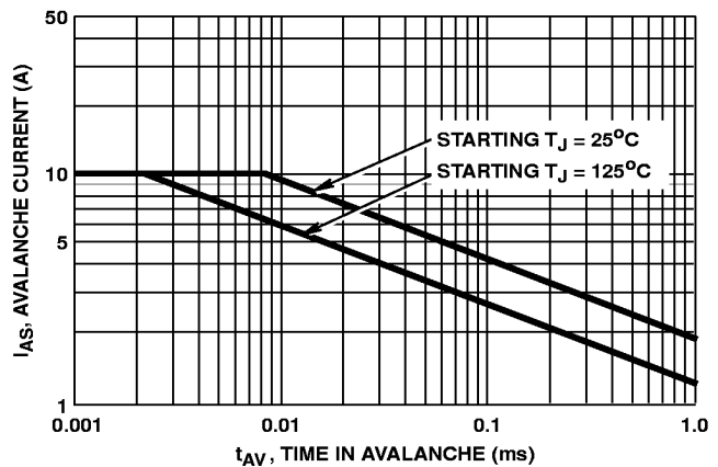
FIGURE 2. UNCLAMPED INDUCTIVE-SWITCHING
