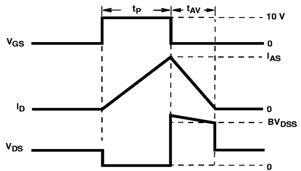
FIGURE 13. UNCLAMPED ENERGY WAVEFORMS
