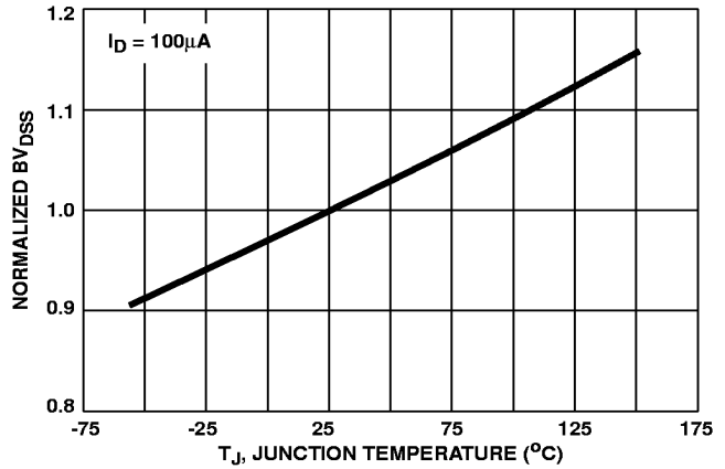
FIGURE 6. NORMALIZED BV_{DS} vs JUNCTION TEMPERATURE
