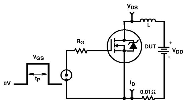
FIGURE 12. UNCLAMPED ENERGY TEST CIRCUIT
