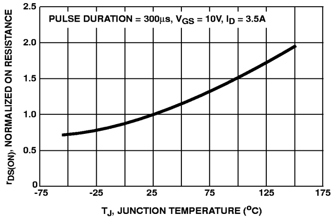
FIGURE 5. NORMALIZED r_{DS(ON)} vs JUNCTION TEMPERATURE
