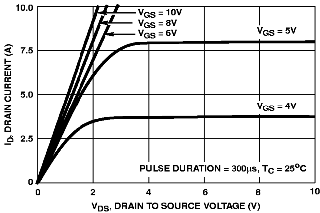
FIGURE 3. TYPICAL SATURATION CHARACTERISTICS
