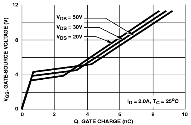
FIGURE 8. GATE-SOURCE VOLTAGE vs GATE CHARGE
