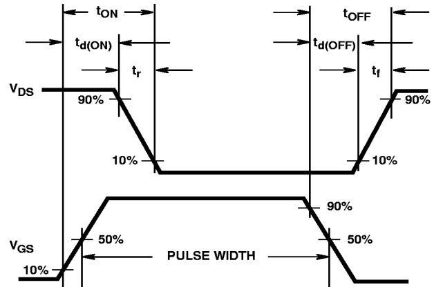
FIGURE 15. RESISTIVE SWITCHING WAVEFORMS
