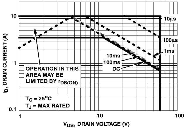
FIGURE 1A. 25^\circ\text{C} SAFE-OPERATING AREA CURVE
