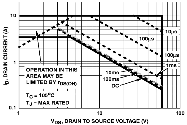
FIGURE 1B. 105^\circ\text{C} SAFE-OPERATING AREA CURVE
