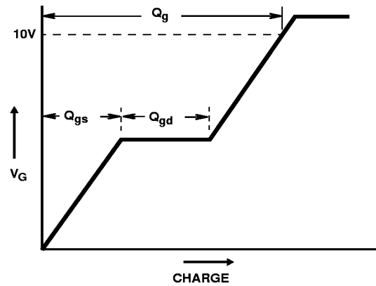
FIGURE 17. BASIC GATE CHARGE WAVEFORM
