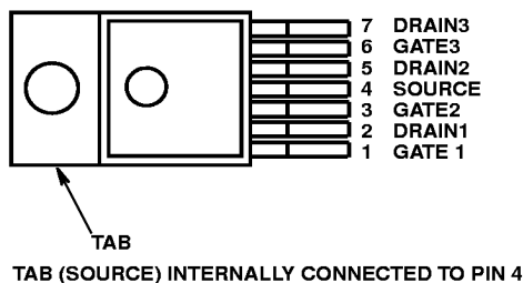
HIP0061AS1 (SIP - VERTICAL) TOP VIEW
