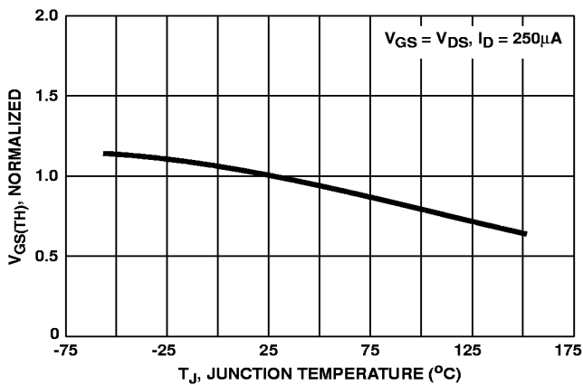
FIGURE 7. NORMALIZED V_{GS(TH)} vs JUNCTION TEMPERATURE
