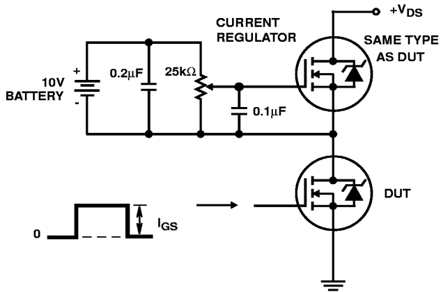
FIGURE 16. GATE CHARGE TEST CIRCUIT
