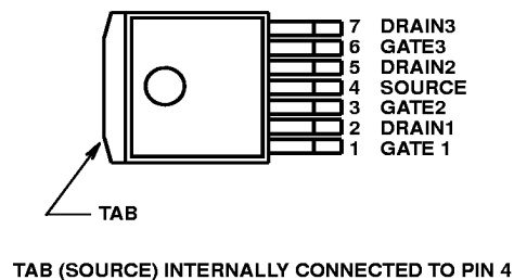
HIP0061AS2 (SIP - GULLWING) TOP VIEW
