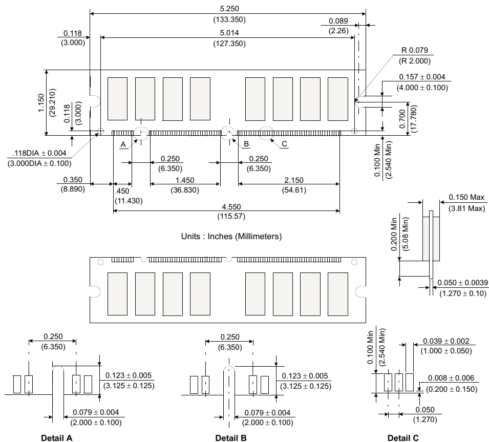
Figure 1: KVR133X64C3/1G 168-Pin SDRAM Module
