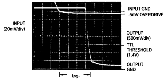
MAX907/MAX908 PROPAGATION DELAY ( t_{PD-} ) (5mV OVERDRIVE)
