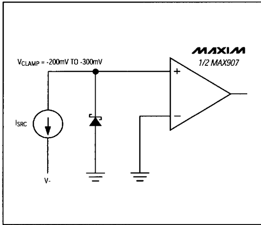
Figure 3. Schottky Clamp for Input Driven Below Ground
