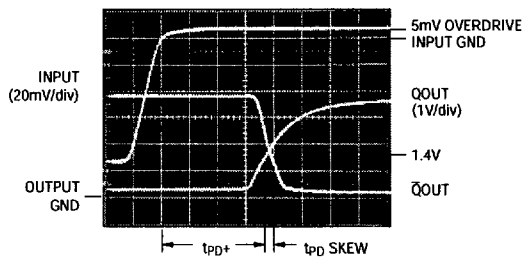
MAX909 PROPAGATION DELAY ( t_{PD+} ) (5mV OVERDRIVE)
