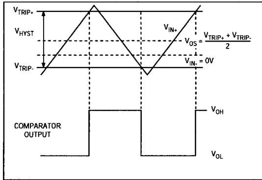
Figure 1. Input and Output Waveforms, Noninverting Input Varied
