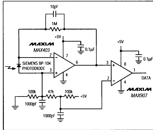
Figure 4. Battery-Operated Infrared Data Link Consumes Only 1mA
