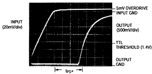
MAX907/MAX908 PROPAGATION DELAY ( t_{PD+} ) (5mV OVERDRIVE)
