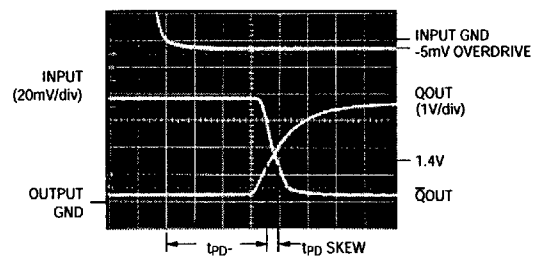
MAX909 PROPAGATION DELAY ( t_{PD-} ) (5mV OVERDRIVE)
