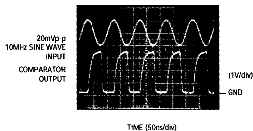
RESPONSE TO 10MHz SINE WAVE
