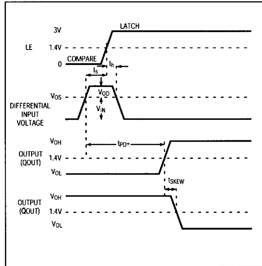
Figure 2. MAX909 Timing Diagram
