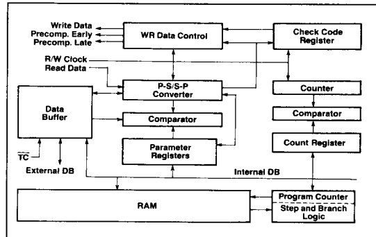
Figure 4. Block Diagram of the Format Controller
