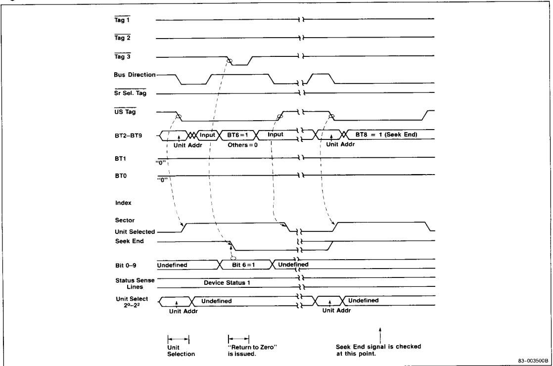
Figure 12. Return to Zero Timing (Hard Sector)
