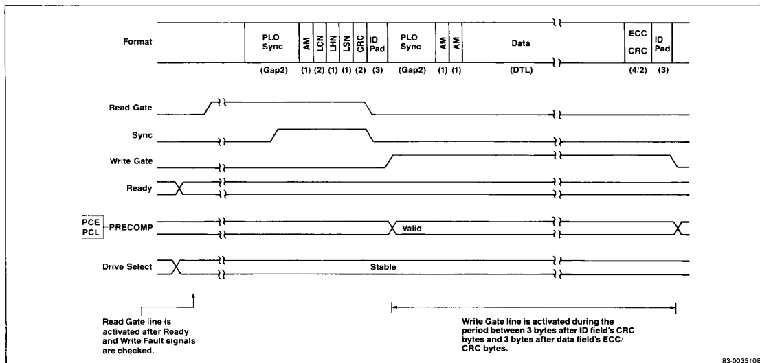
Figure 22. "Data Write" Timing (Soft Sector)
