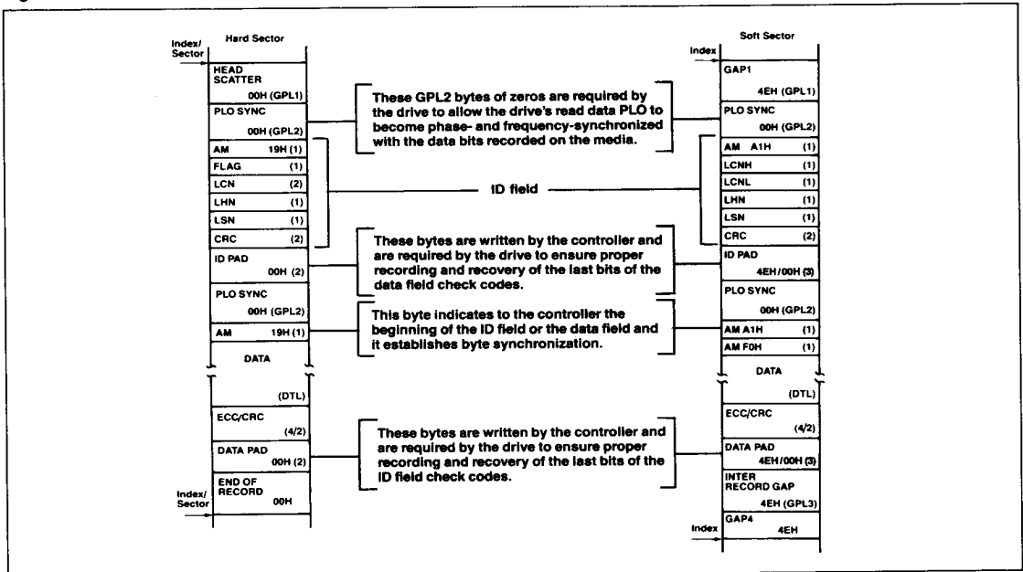
Figure 10. Track Format
