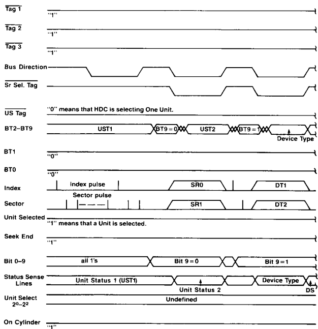
Figure 15. "Unit Status Sense" Timing (Hard Sector)
