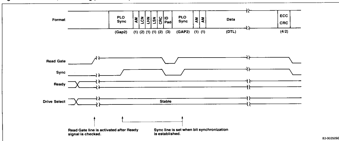
Figure 21. "Data Read" Timing (Soft Sector)
