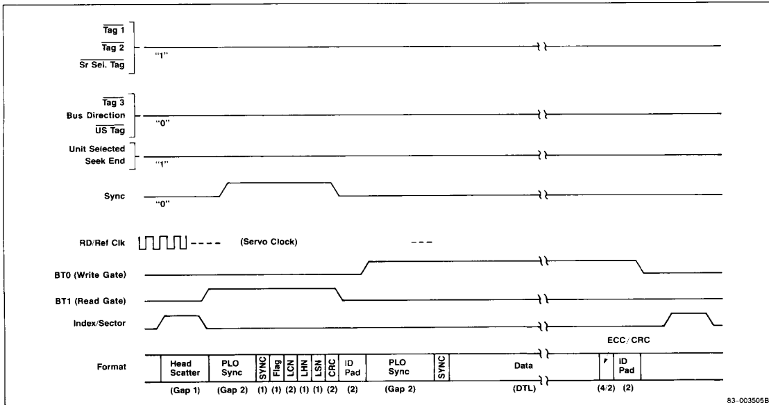
Figure 17. "Data Write" Timing (Hard Sector)
