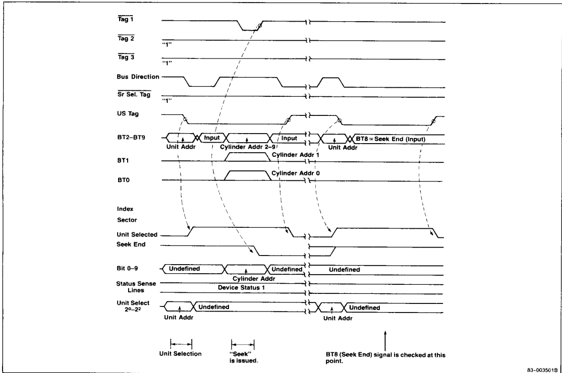
Figure 13. "Seek" Timing (Hard Sector)
