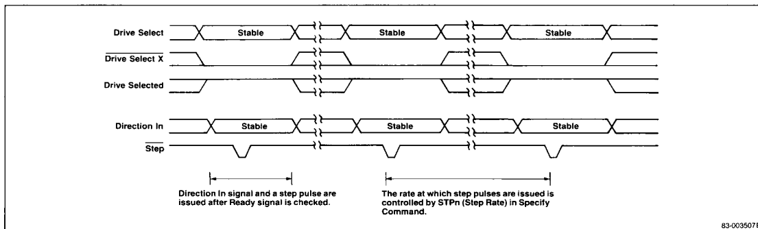
Figure 19. "Normal Seek" Timing (Soft Sector)
