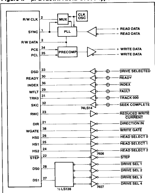
Figure 1. μPD7261A/7261B ST506-Type Interface
