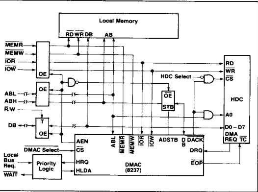
Figure 9. Local Bus System
