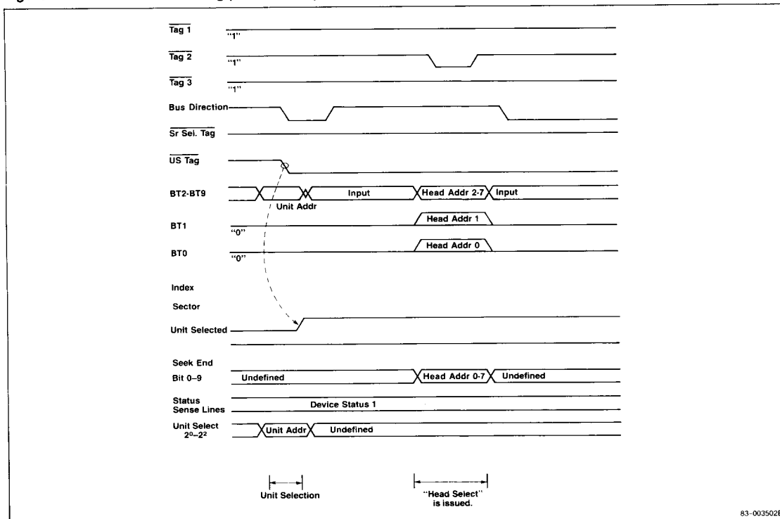
Figure 14. "Head Select" Timing (Hard Sector)
