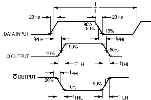
Figure 1. AC and Power Dissipation Test Circuit and Timing Diagram (Data to Output)
