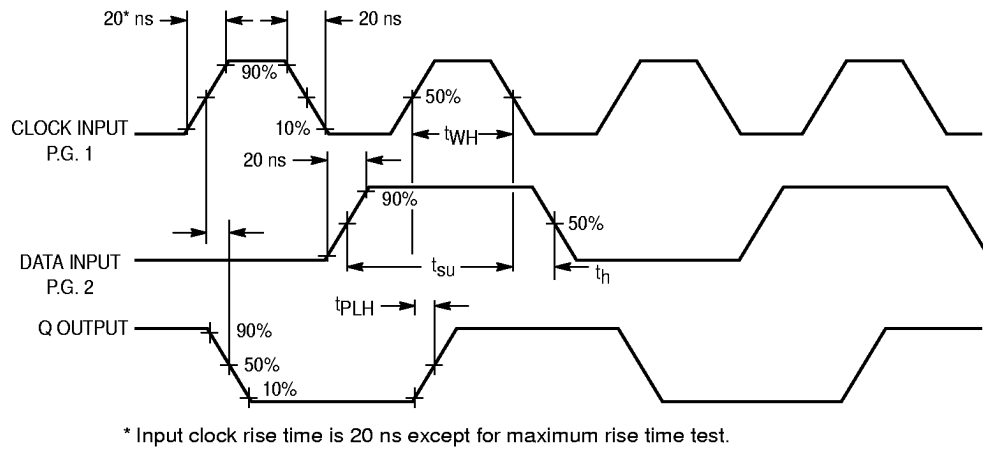
Figure 2. AC Test Circuit and Timing Diagram (Clock to Output)
