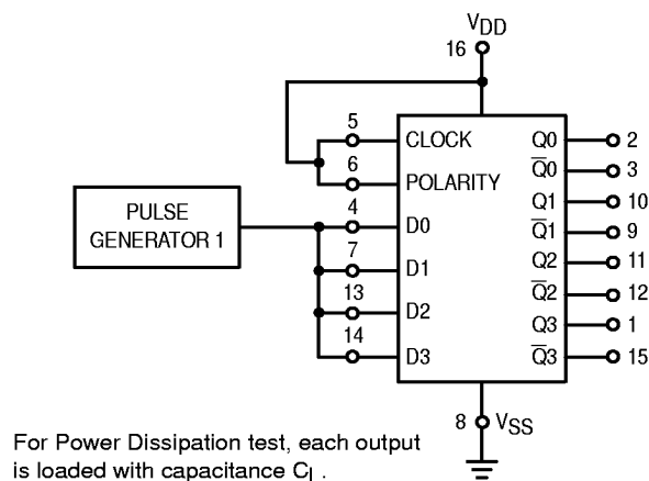
Figure 1. AC and Power Dissipation Test Circuit and Timing Diagram (Data to Output)
