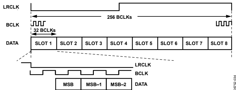
Figure 34. TDM Mode
