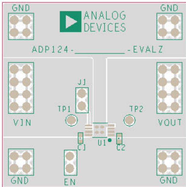
Figure 41. Example ADP124 PCB Layout
