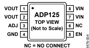
Figure 4. ADP125 Adjustable Output Pin Configuration
