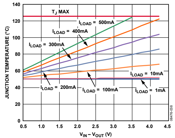
Figure 38. Junction Temperature vs. Power Dissipation, 500 mm 2 of PCB Copper, T_A = 50^\circ\text{C}
