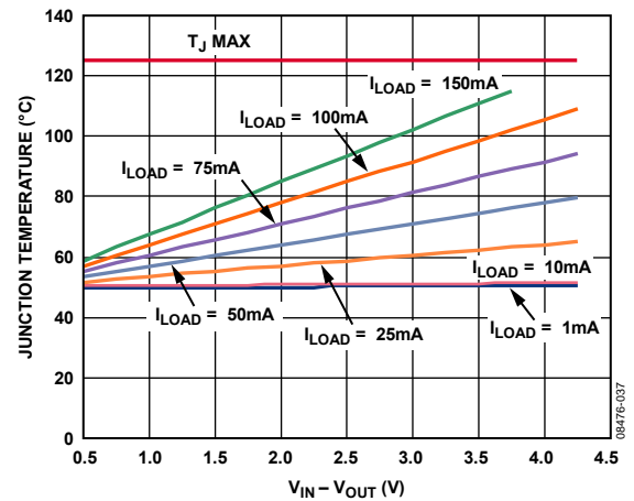
Figure 37. Junction Temperature vs. Power Dissipation, 1000 mm 2 of PCB Copper, T_A = 50^\circ\text{C}
