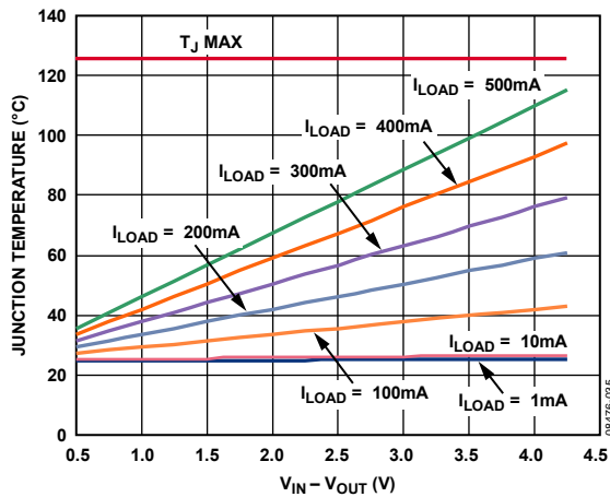
Figure 35. Junction Temperature vs. Power Dissipation, 500 mm 2 of PCB Copper, T_A = 25^\circ\text{C}
