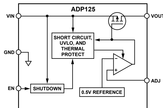
Figure 27. ADP125 Internal Block Diagram (Adjustable Output)
