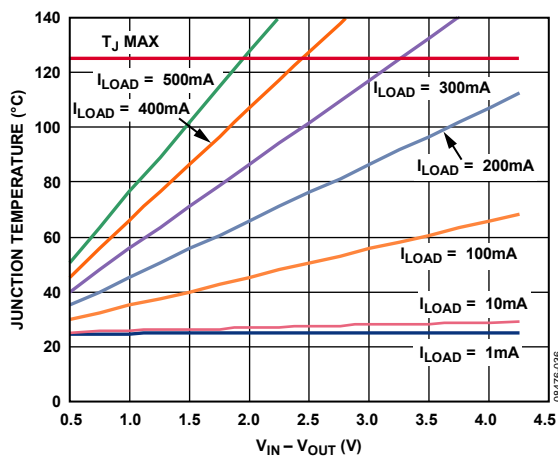
Figure 36. Junction Temperature vs. Power Dissipation, 40 mm 2 of PCB Copper, T_A = 25^\circ\text{C}
