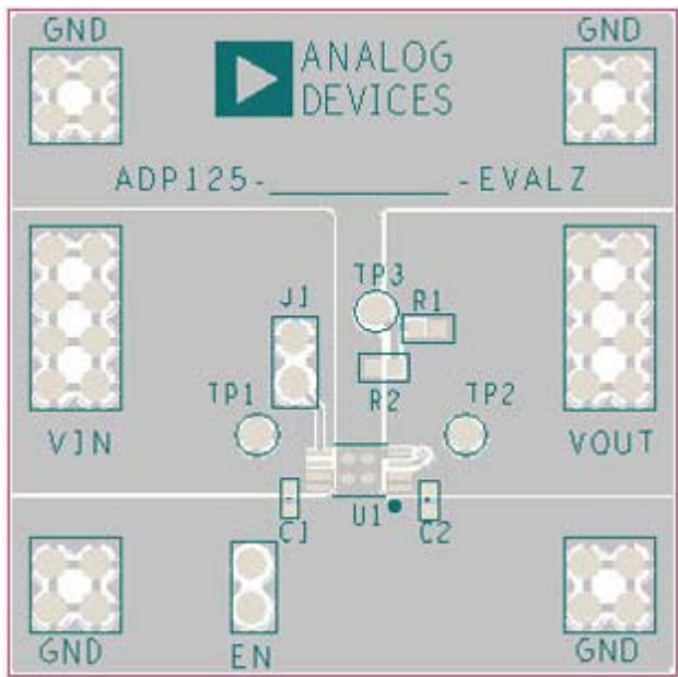
Figure 42. Example ADP125 PCB Layout
