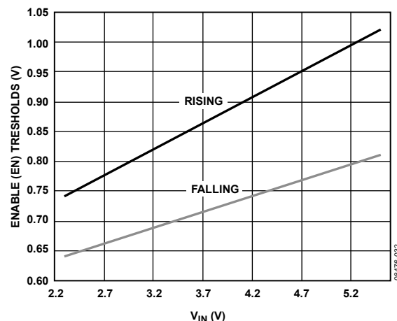
Figure 32. Typical EN Pin Thresholds vs. Input Voltage
