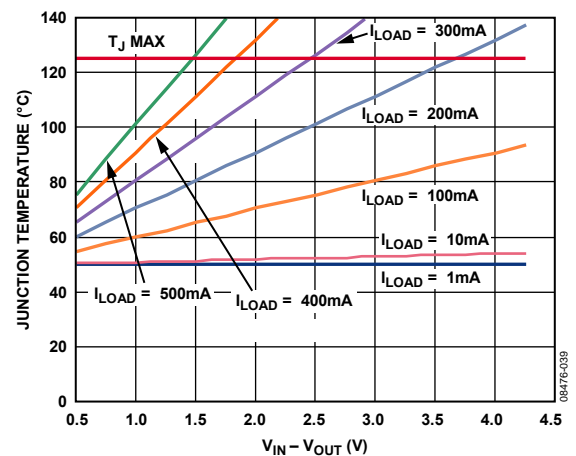
Figure 39. Junction Temperature vs. Power Dissipation, 40 mm 2 of PCB Copper, T_A = 50^\circ\text{C}
