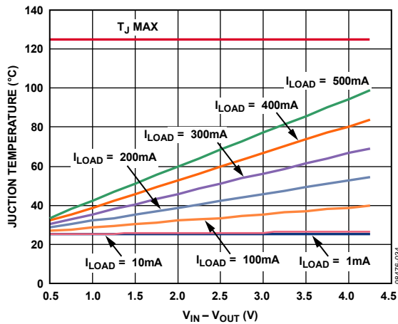
Figure 34. Junction Temperature vs. Power Dissipation, 1000 mm 2 of PCB Copper, T_A = 25^\circ\text{C}
