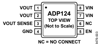
Figure 3. ADP124 Fixed Output Pin Configuration
