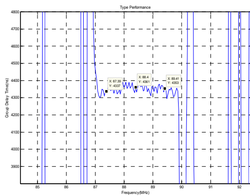
Group Delay Variation (f0±1MHz)
