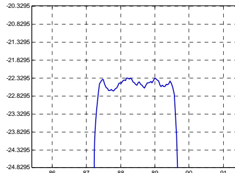
Passband Response
