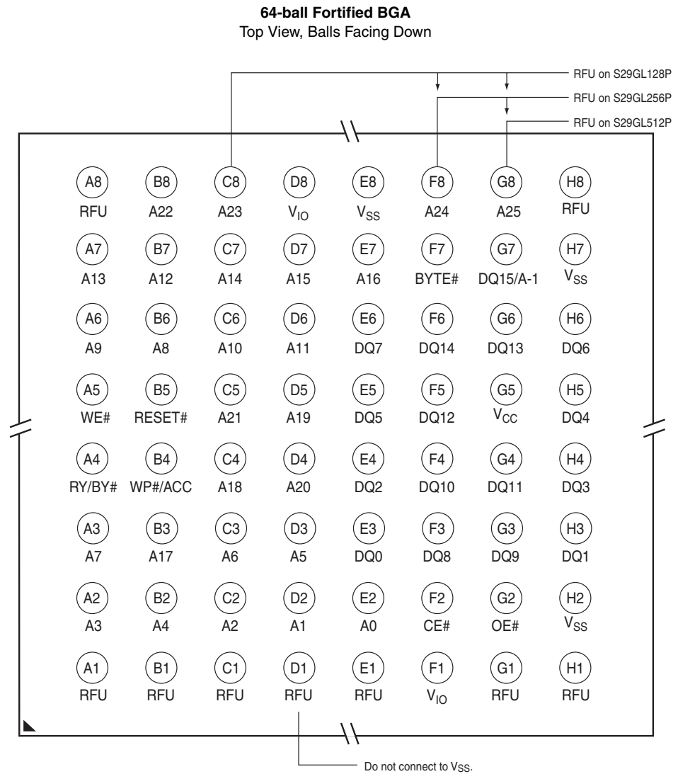
Figure 4.1 64-ball Fortified Ball Grid Array
