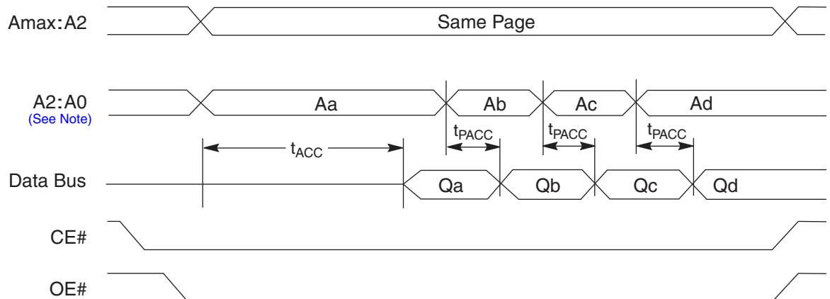
Figure 11.6 Page Read Timings
