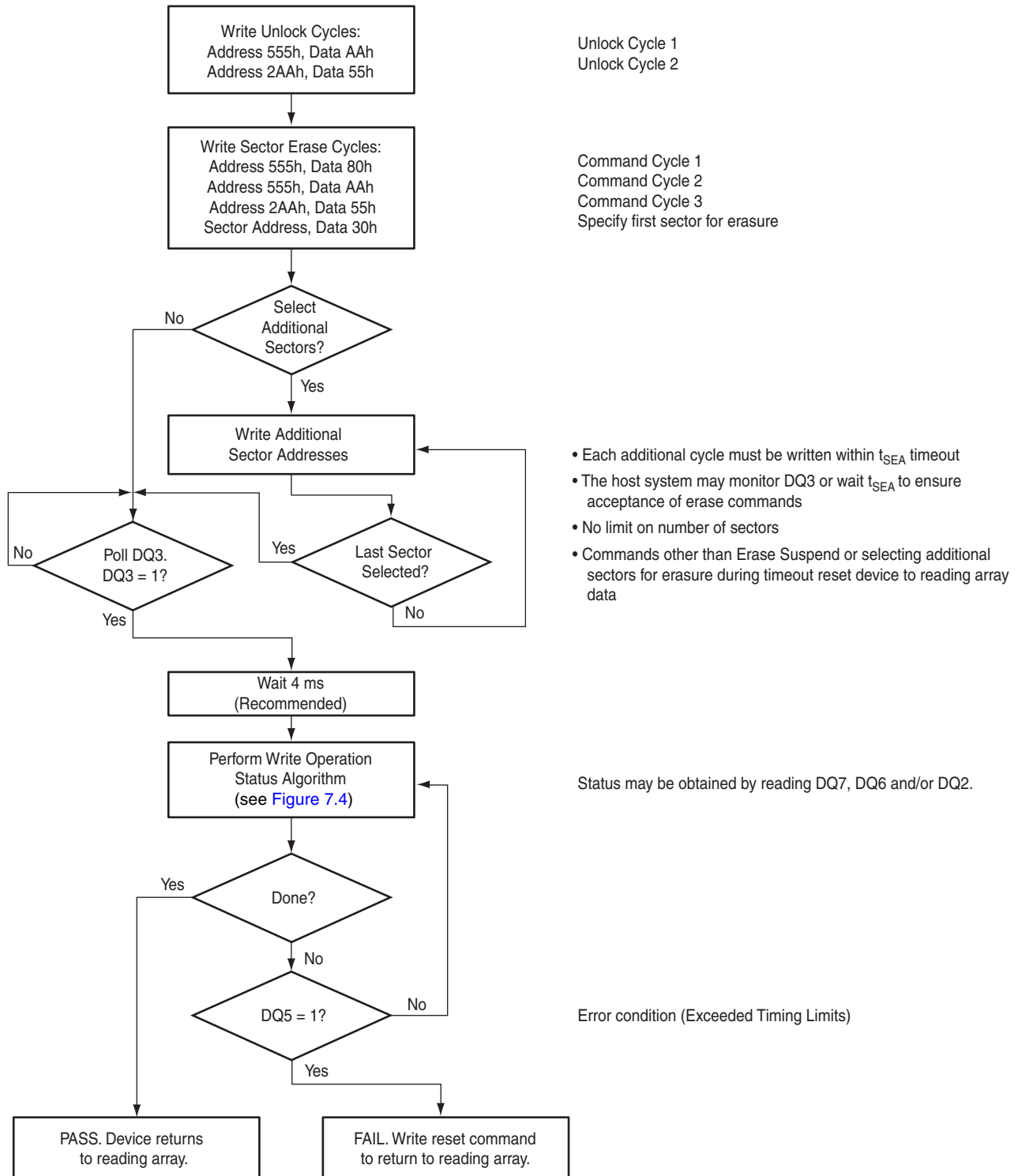
Figure 7.3 Sector Erase Operation
