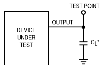
Figure 2. Test Circuit
