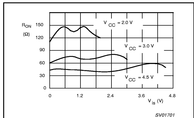
Figure 4. Typical ON-resistance ( R_{on} ) as a function of input voltage ( V_{is} ) for V_{is} = 0 \text{ to } V_{CC} - V_{EE} .
