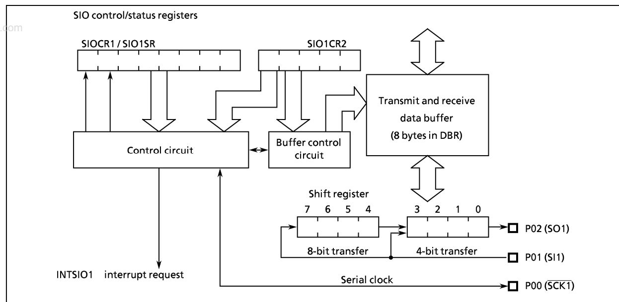
Figure 2-63. Serial Interfaces
