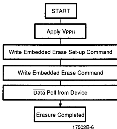
Figure 5. Embedded Erase Algorithm
