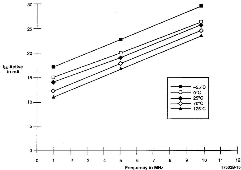
Figure 9. Am28F020A - Average I_{cc} Active vs. Frequency V_{cc} = 5.5 V, Addressing Pattern = Minimax Data Pattern = Checkerboard
