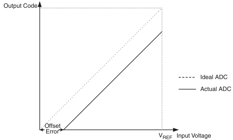
Figure 20-10. Offset Error
