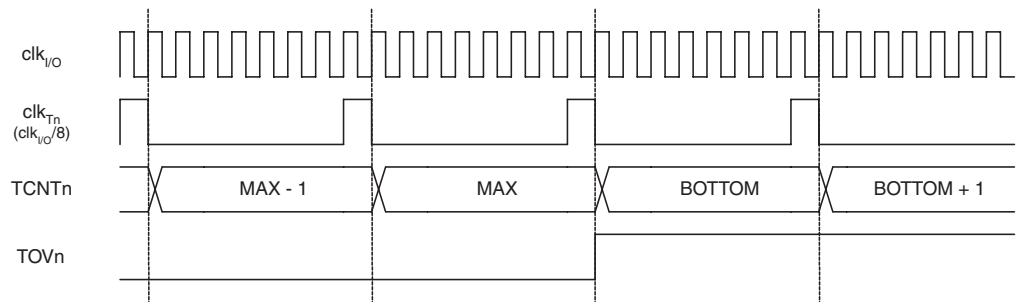
Figure 5. Timer/Counter Timing Diagram, with Prescaler ( f_{clk\_I/O}/8 )
