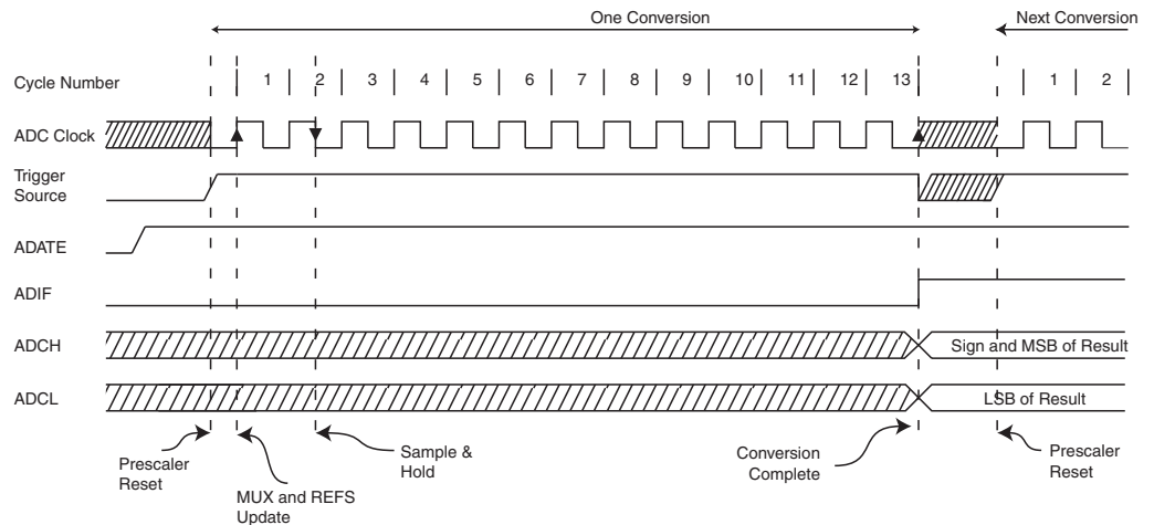
Figure 20-6. ADC Timing Diagram, Auto Triggerged Conversion
