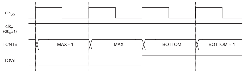
Figure 4. Timer/Counter Timing Diagram, no Prescaling
