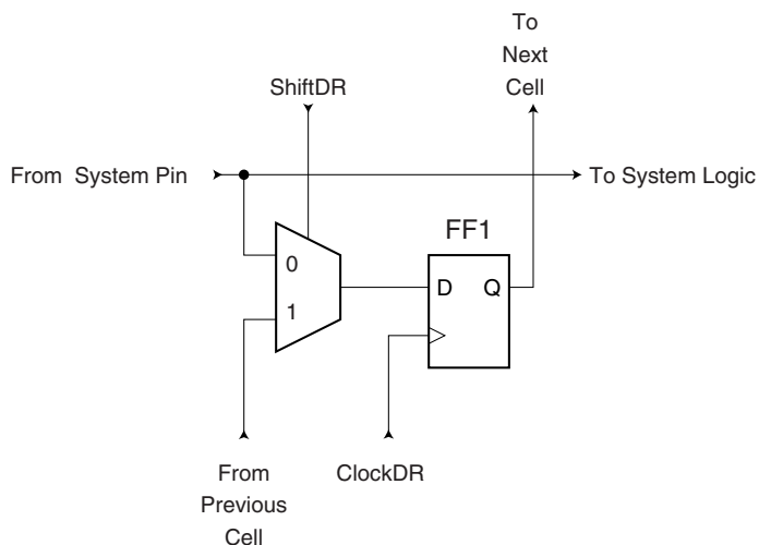
Figure 22-4. Observe-only Cell
