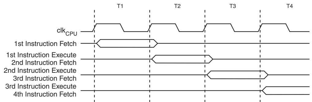
Figure 1. The Parallel Instruction Fetches and Instruction Executions
