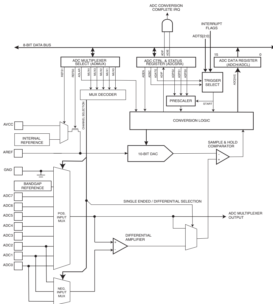
Figure 20-1. Analog to Digital Converter Block Schematic
