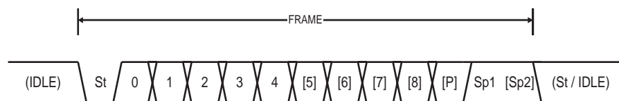
Figure 17-5. Frame Formats
