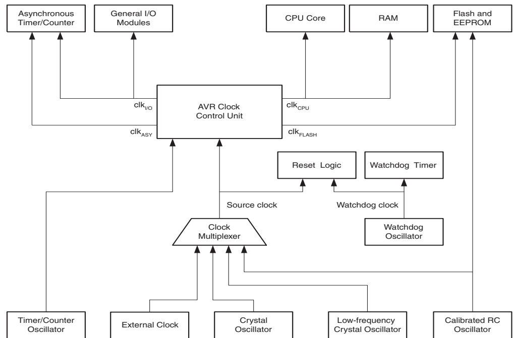
Figure 7-1. Clock Distribution
