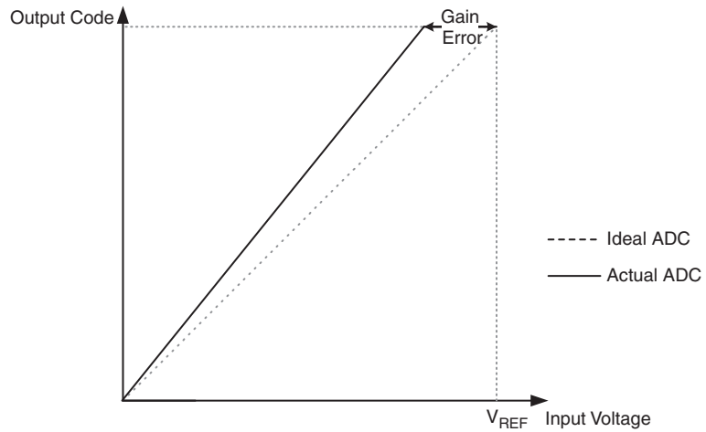
Figure 20-11. Gain Error
