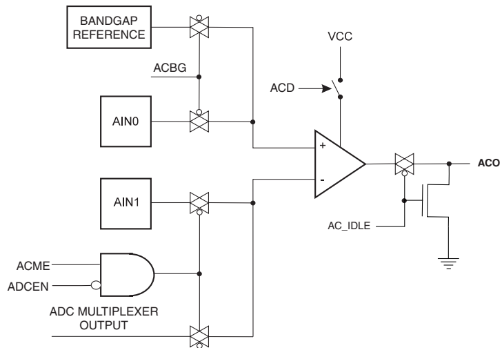
Figure 22-6. Analog Comparator
