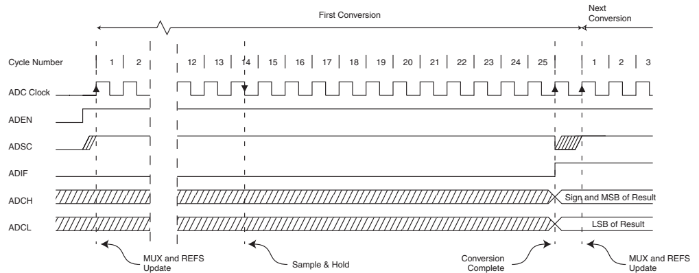
Figure 20-4. ADC Timing Diagram, First Conversion (Single Conversion Mode)
