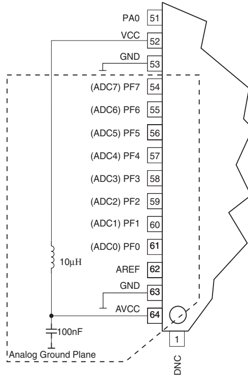
Figure 20-9. ADC Power Connections
