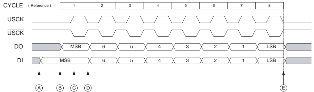
Figure 18-3. Three-wire Mode, Timing Diagram
