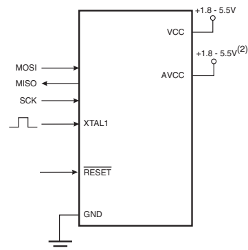
Figure 24-10. Serial Programming and Verify (1)
