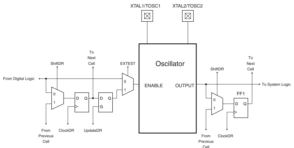
Figure 22-5. Boundary-scan Cells for Oscillators and Clock Options
