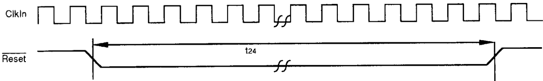
Figure 10. Warm Reset Sequence
