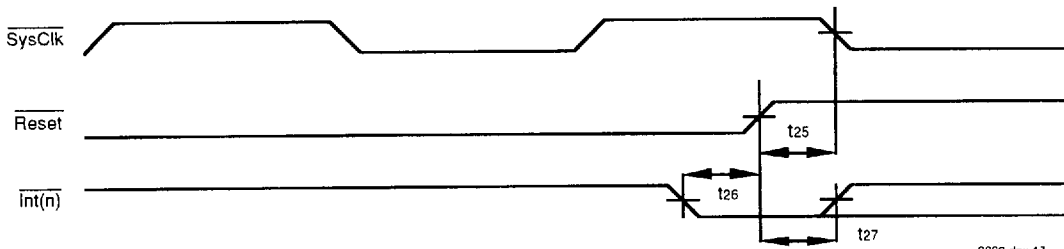
Figure 11. Mode Selection and Negation of Reset
