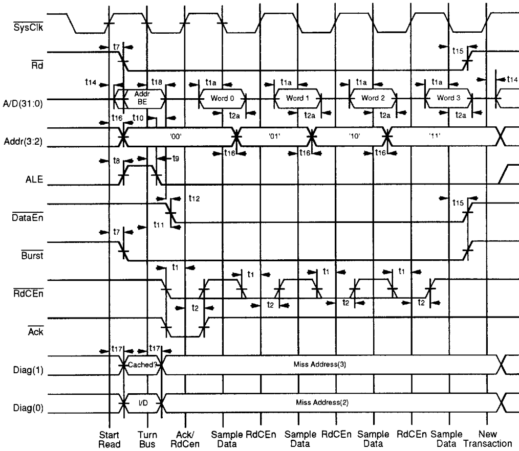
Figure 13. R3081 Burst Read
