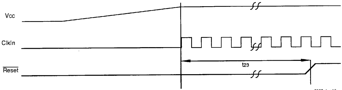
Figure 9. Power-On Reset Sequence
