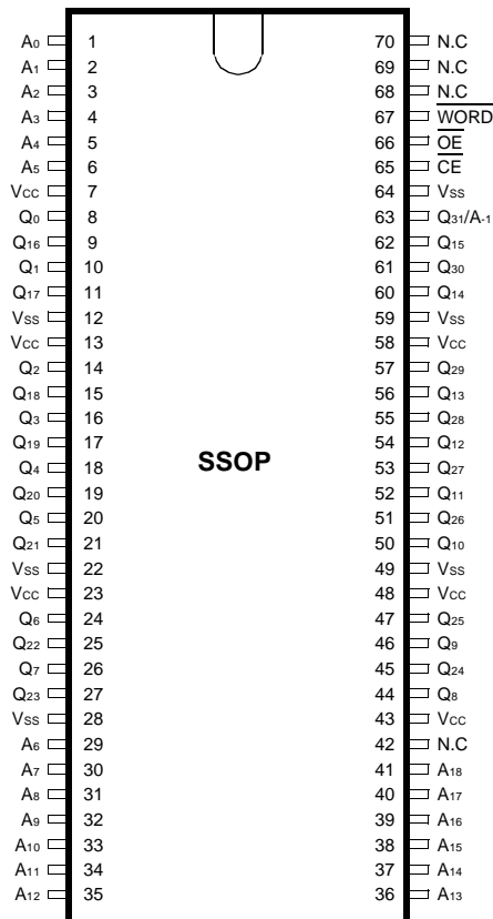
K3P5C2000D-SC
