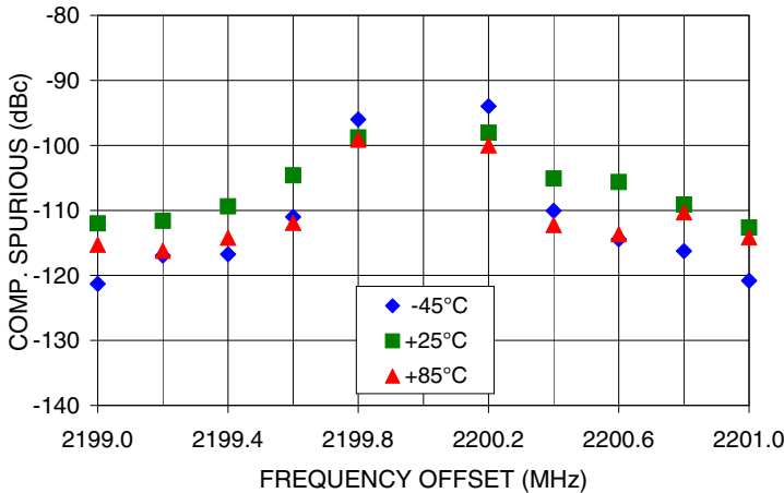
COMPARISON SPURIOUS Vs FREQ. OFFSET @ Fcar = 2200MHz
