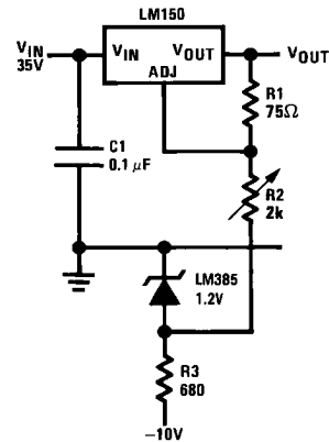
0 to 30V Regulator
