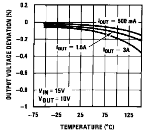
Load Regulation
